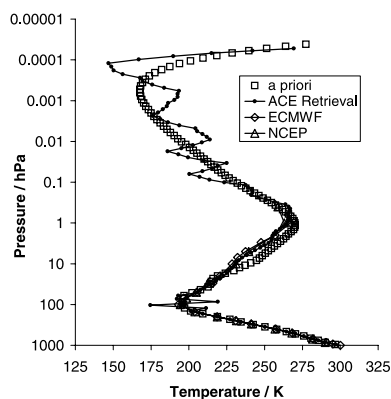
Figure 3. Comparison of the ACE-FTS a priori T versus p with the retrieved result and weather forecast models.
