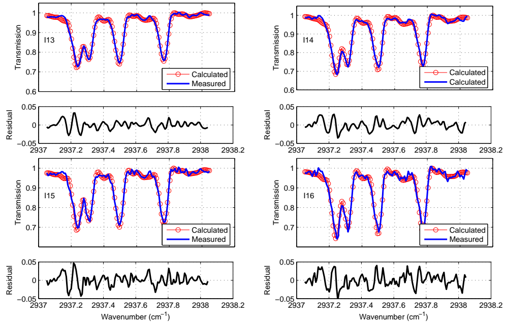
Figure 5.14: As in Figure 5.6, but for InSb CH 4 spectral fits.
