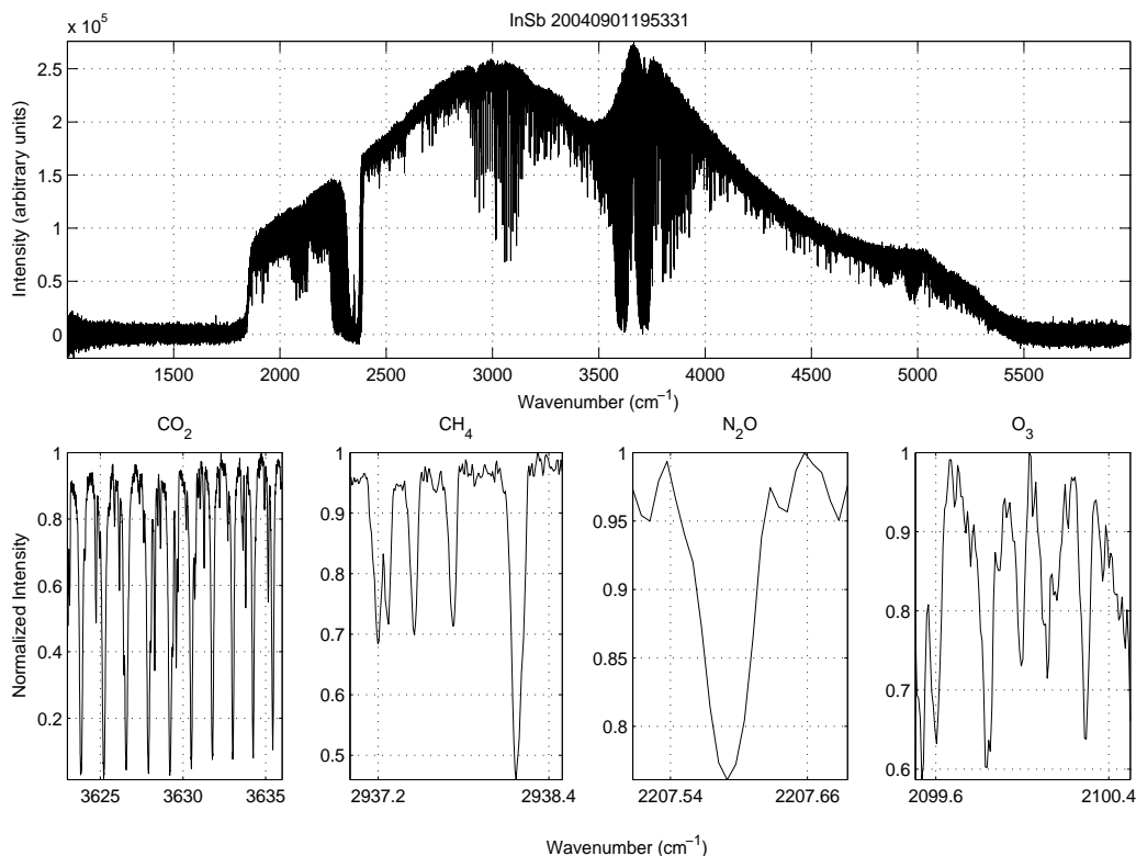
Figure 4.11: InSb spectrum from MANTRA 2004 flight 1
