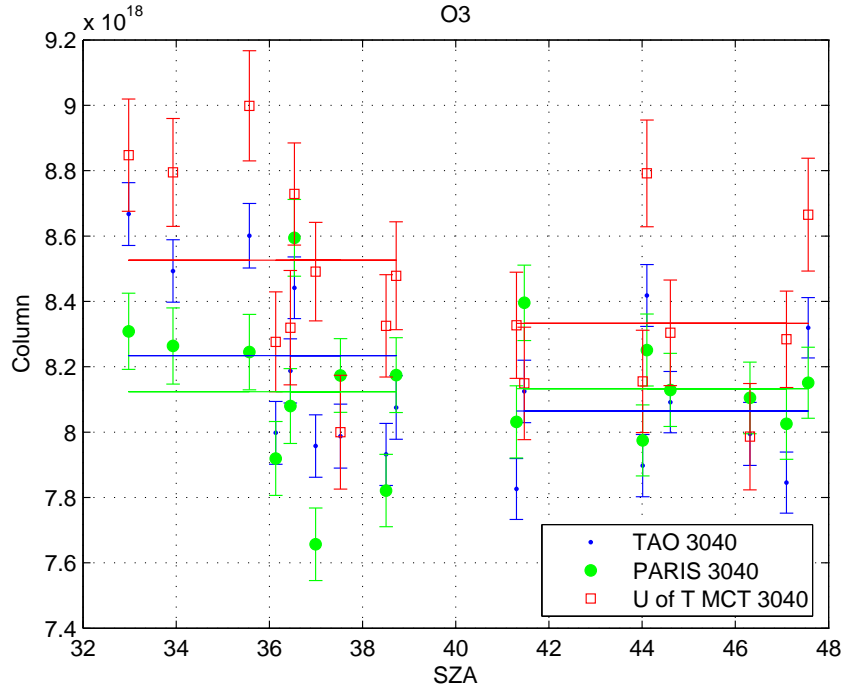
Figure 5.56: O 3 column amounts retrieved in the 3040 cm -1 microwindow as a function of solar zenith angle, using the parameters listed in Table 5.13. The horizontal lines show the means of the columns over the SZA range indicated. The error bars include the smoothing error, interference error, and the retrieval error added in quadrature.
