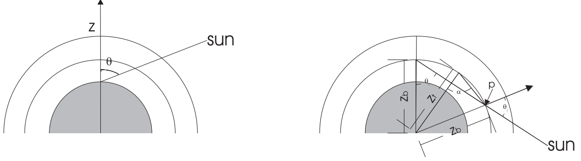
Figure 1.3: Ground-based (left panel) and balloon-based (right panel) viewing geometries.
