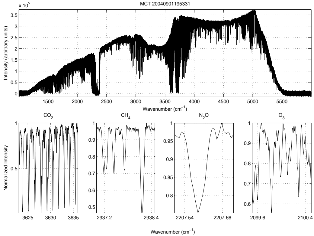
Figure 4.12: MCT spectrum from MANTRA 2004 flight 1
