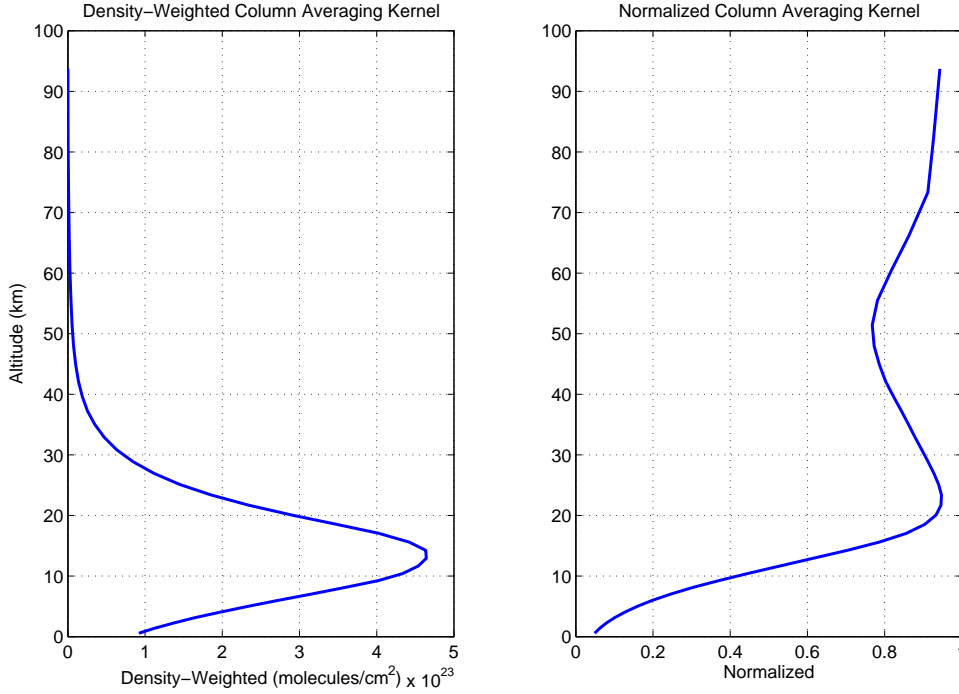
Figure 5.1: Density-weighted and normalized column averaging kernels for a typical ozone profile in the 3040\text{ cm}^{-1} microwindow for the U of T FTS MCT detector.
