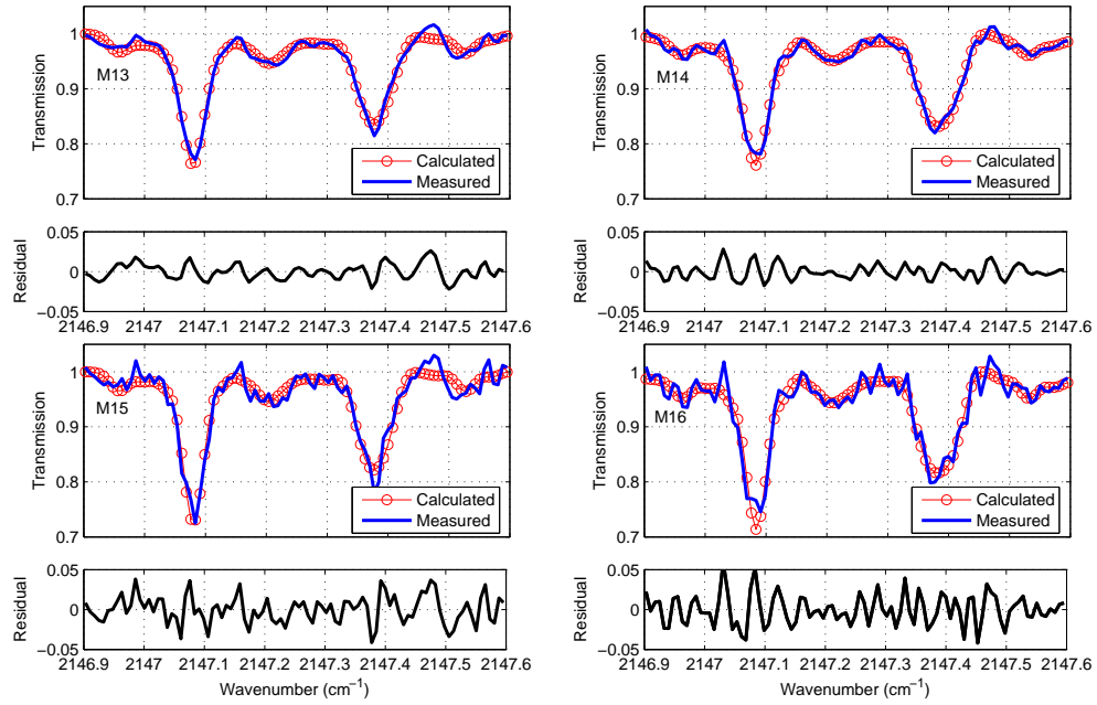
Figure 5.13: As in Figure 5.6, but for MCT CO spectral fits.
