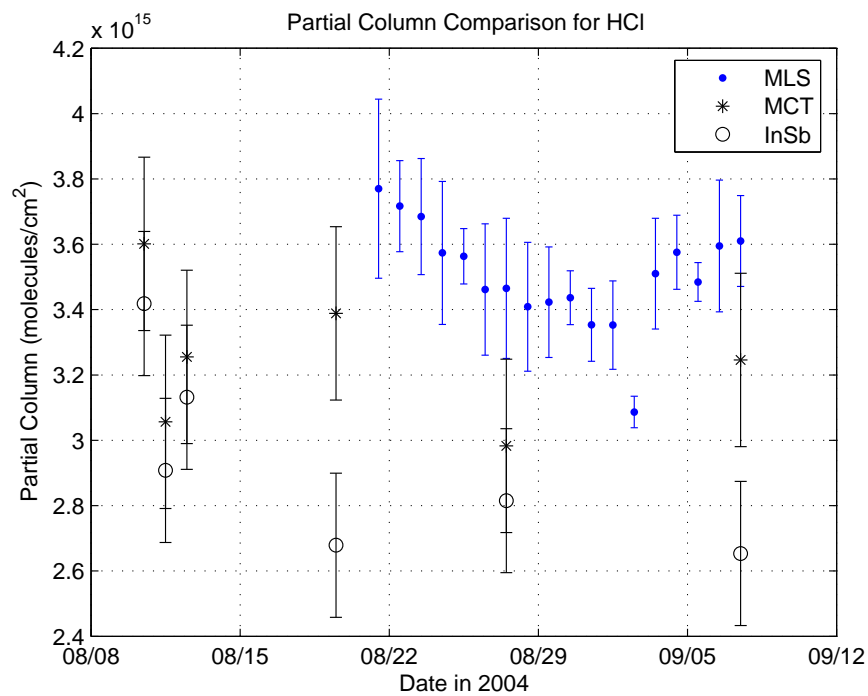
Figure 5.30: HCl partial column comparisons with MLS.
