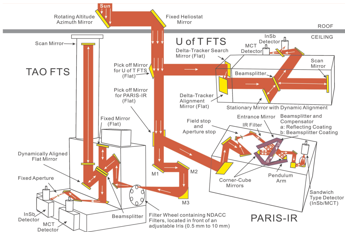
Figure 5.35: The experimental setup. Figure courtesy Dejian Fu.
