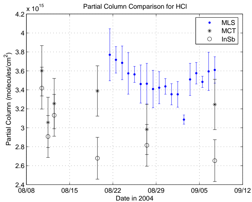
Figure 5.28: HCl partial column comparisons with MLS.
