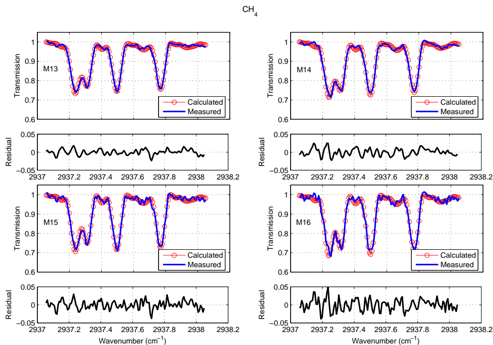
Figure 5.13: As in Figure 5.4, but for MCT \text{CH}_4 spectral fits.
