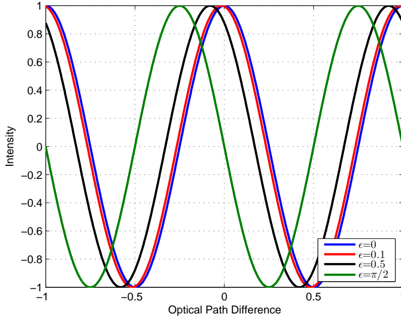
Figure 3.5: Cosine interferogram with different phase errors, \epsilon .
