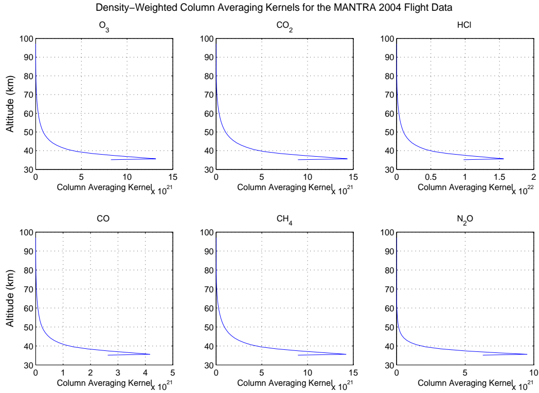
Figure 5.3: Flight column averaging kernels.
