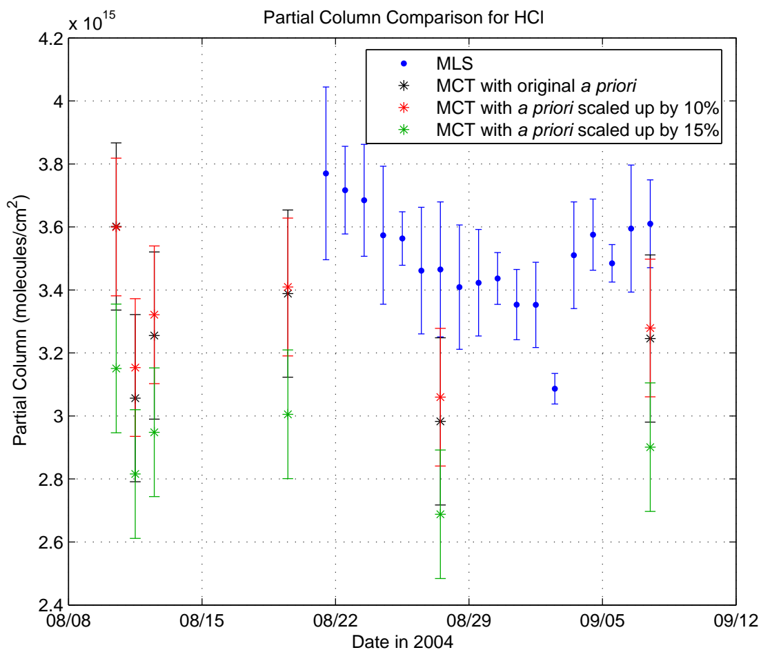
Figure 5.29: HCl partial column comparisons with MLS. The different colours for the U of T FTS partial column data correspond to the different a priori profiles used to retrieve HCl partial columns, in an attempt to improve agreement between MLS and the U of T FTS.
