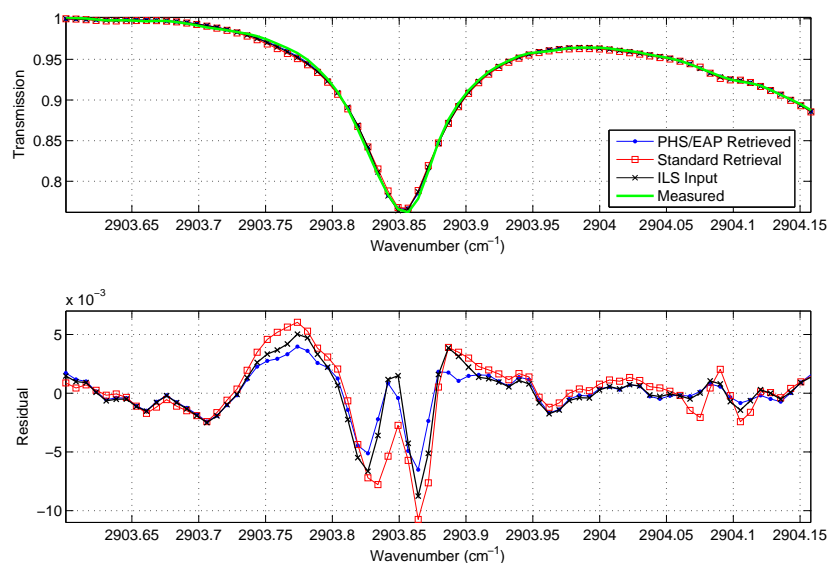
Figure 5.49: CH 4 spectral fits for the third CH 4 bandpass of the U of T FTS (upper panel), and the corresponding residuals (lower panel).
