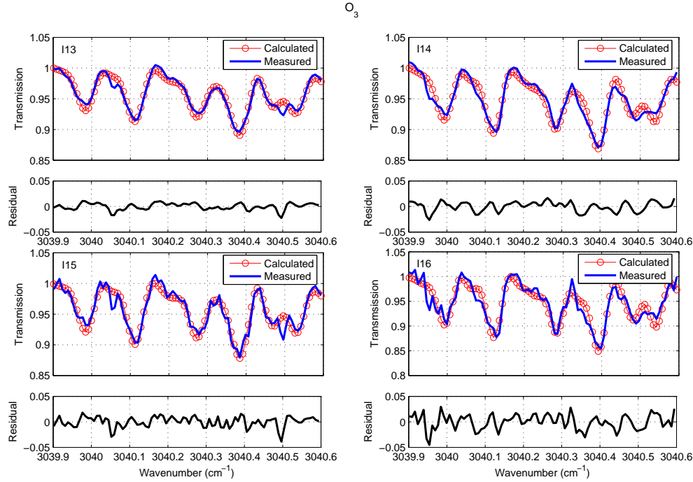
Figure 5.4: Flight data InSb O_3 spectral fits. The four panels show the four spectra described in Table 5.1.
