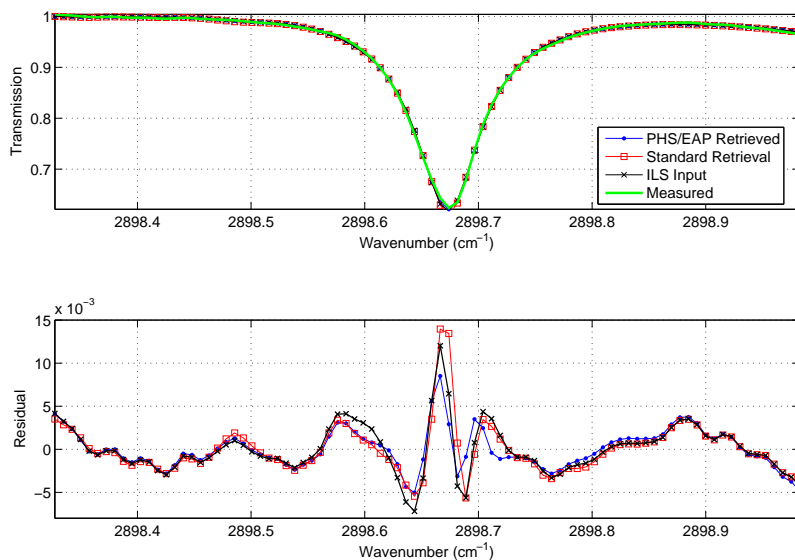
Figure 5.48: CH 4 spectral fits for the second CH 4 bandpass of the U of T FTS (upper panel), and the corresponding residuals (lower panel).
