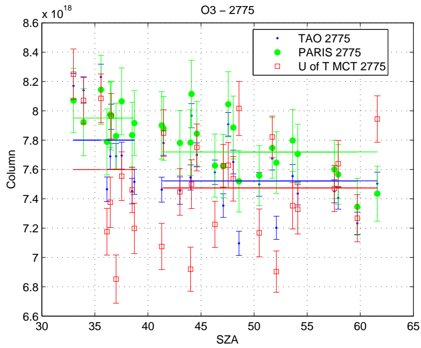
Figure 5.56: As in Figure 5.55, but for O_3 in the 2775\text{ cm}^{-1} microwindow.
