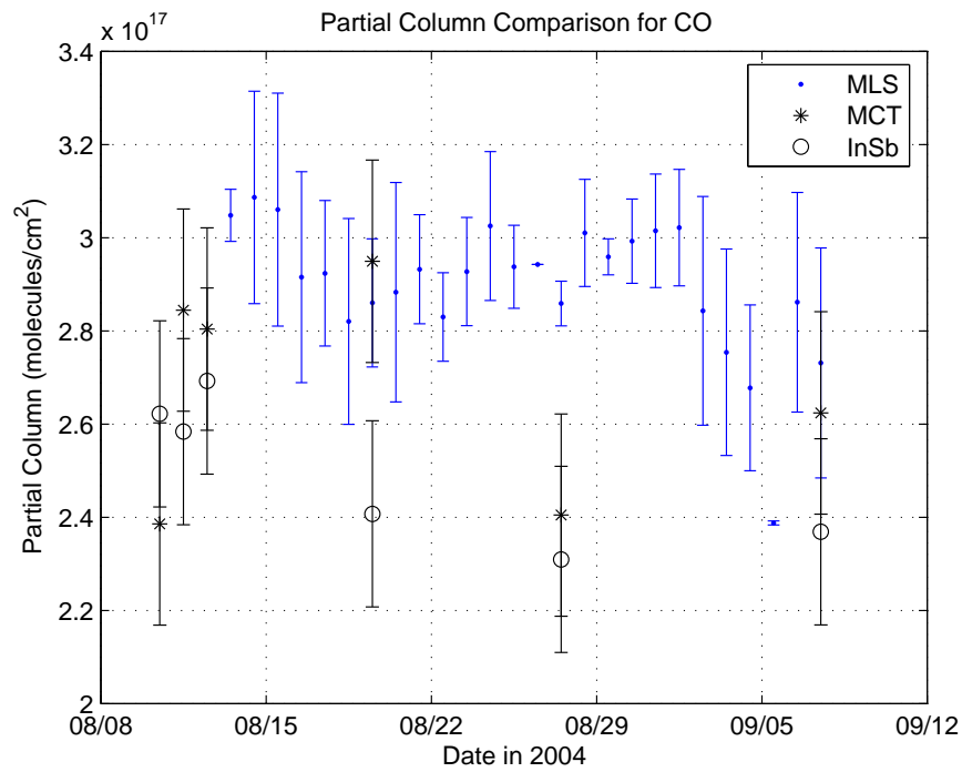
Figure 5.33: CO partial column comparisons with MLS.
