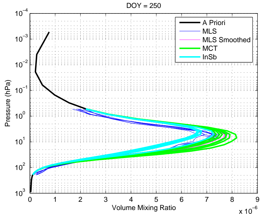
Figure 5.25: Ozone partial profile comparisons with MLS. This figure shows the full a priori profile for the U of T FTS data, with the retrieved U of T FTS and MLS profiles over the appropriate pressure range as defined in Livesey et al. [101].
