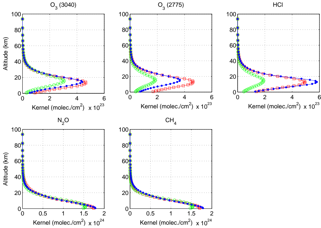
Figure 5.60: Density-weighted column averaging kernels for the three instruments: TAO-FTS (blue dots), U of T FTS (red squares) and the PARIS-IR (green circles), illustrating the sensitivity of the retrieved column at each altitude.
