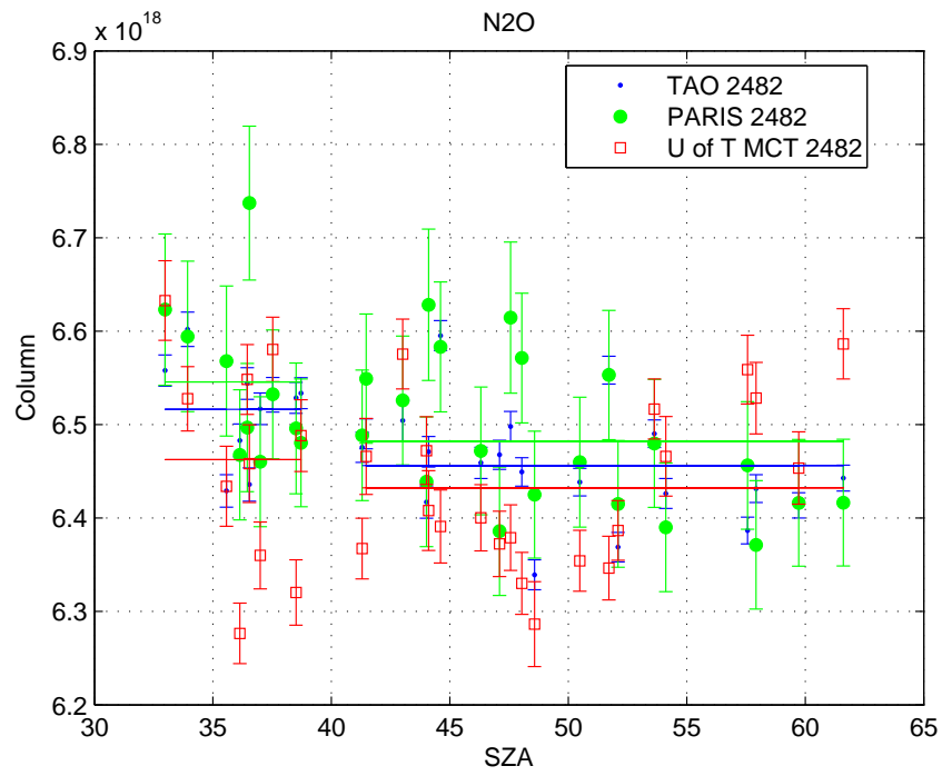
Figure 5.58: As in Figure 5.55, but for \text{N}_2\text{O} .
