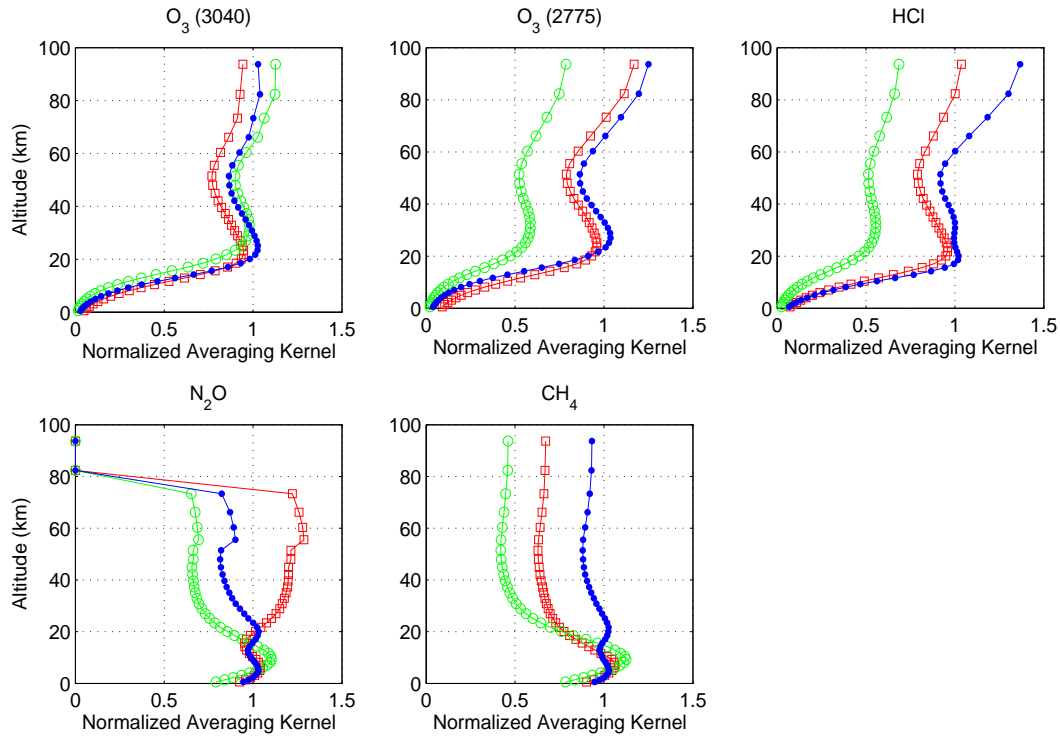
Figure 5.61: Normalized column averaging kernels. These panels show the normalized column averaging kernels for the three instruments: TAO-FTS (blue dots), U of T FTS (red squares) and the PARIS-IR (green circles).
