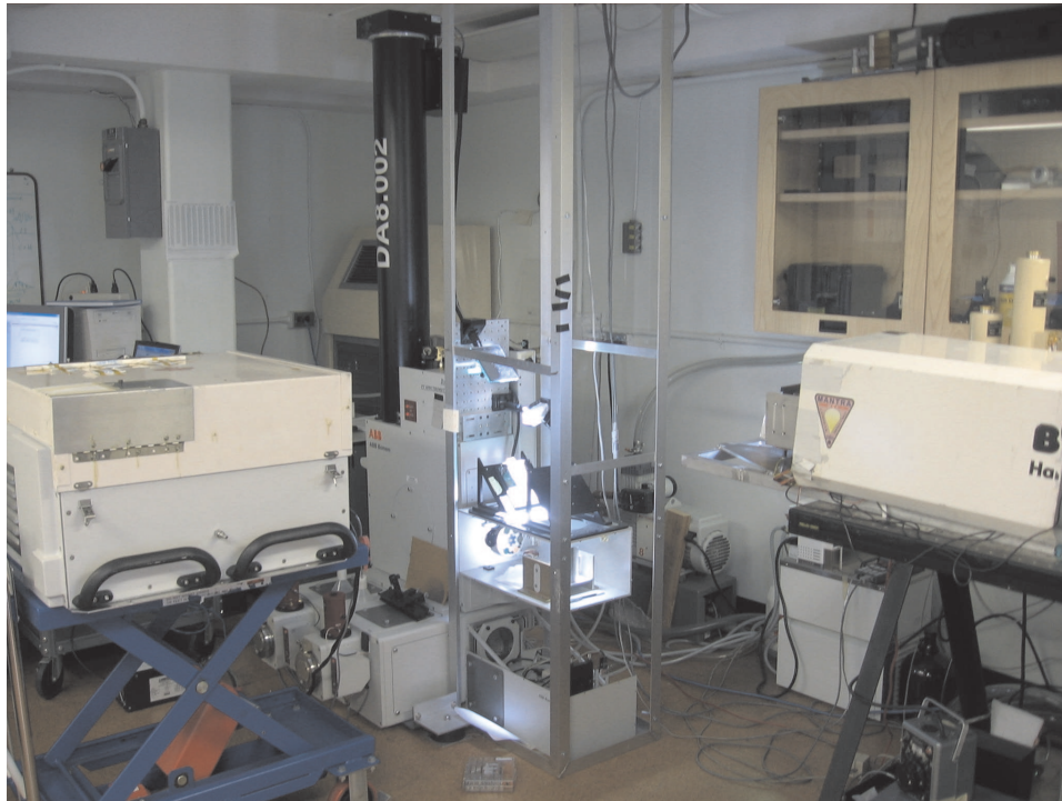
Figure 5.36: Photograph of the experimental setup. The PARIS-IR is on the left of the picture, the U of T FTS is on the right, and the TAO-FTS is located in the centre.
