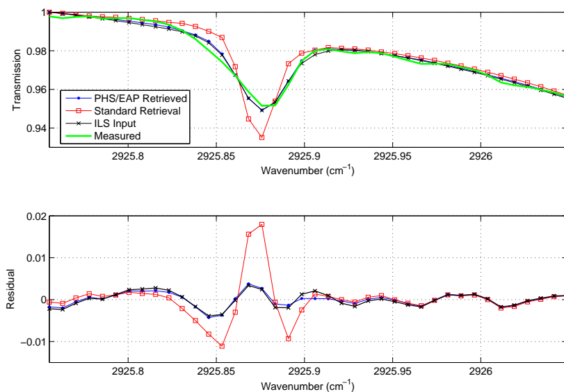
Figure 5.45: HCl spectral fits for the U of T FTS (upper panel), and the corresponding residuals (lower panel).
