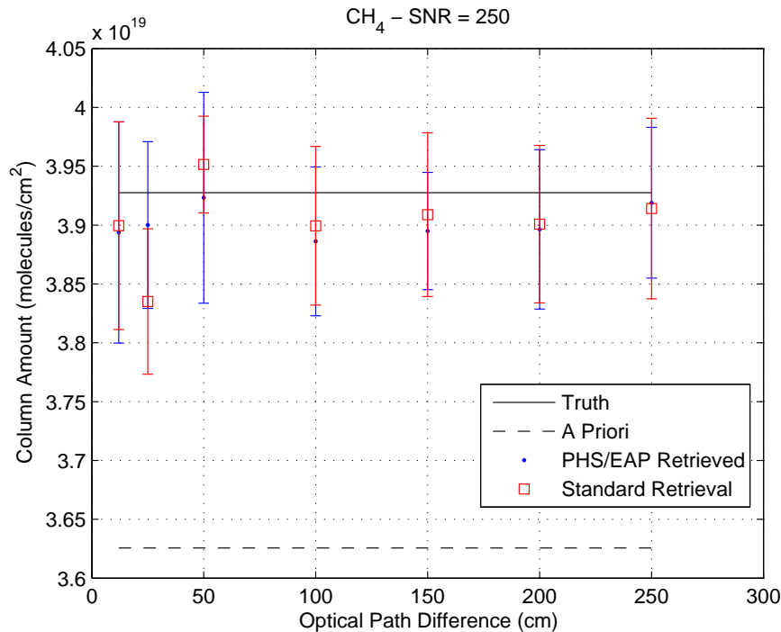
Figure 5.42: Simulated retrievals of \text{CH}_4 columns, assuming \text{SNR}=250 , as a function of OPD.
