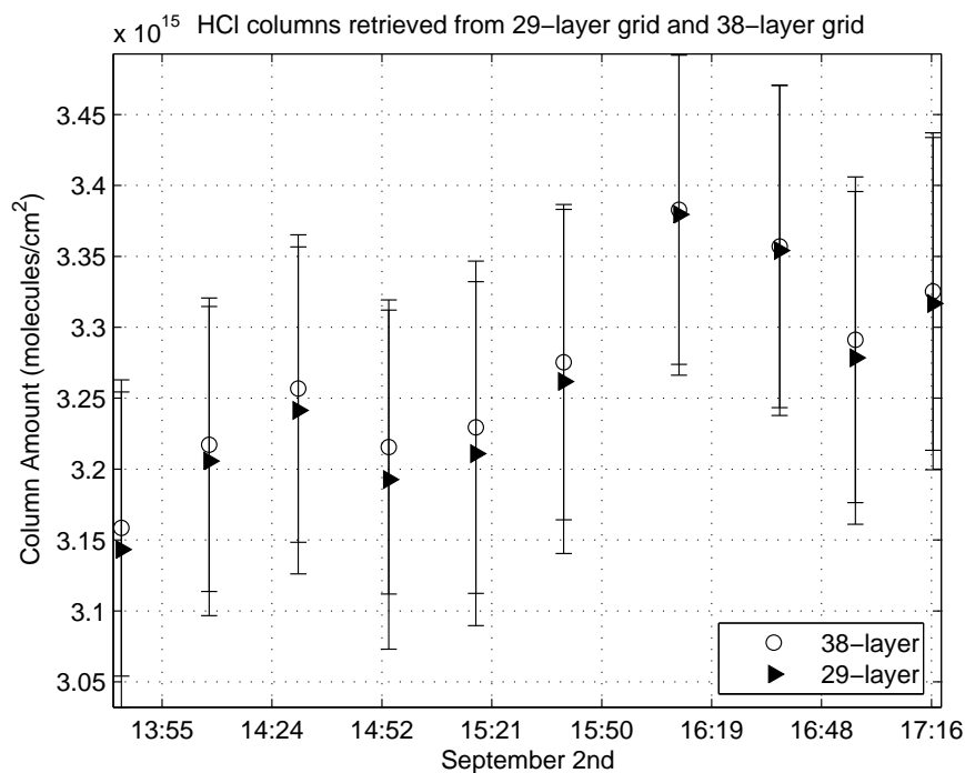
Figure 5.52: \text{HCl} columns retrieved for 38- and 29-grid layers for PARIS-IR.
