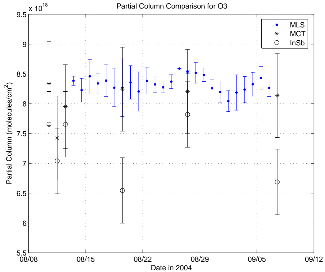
Figure 5.26: Ozone partial column comparisons with MLS.
