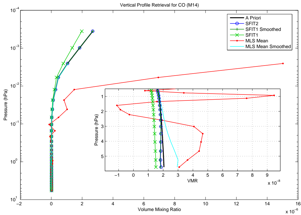
Figure 5.21: The SFIT2 profile, original and smoothed SFIT1 profiles, and original and smoothed MLS mean profiles of CO from the MANTRA 2004 flight data. The inset is an enlargement of the lowest pressure levels.
