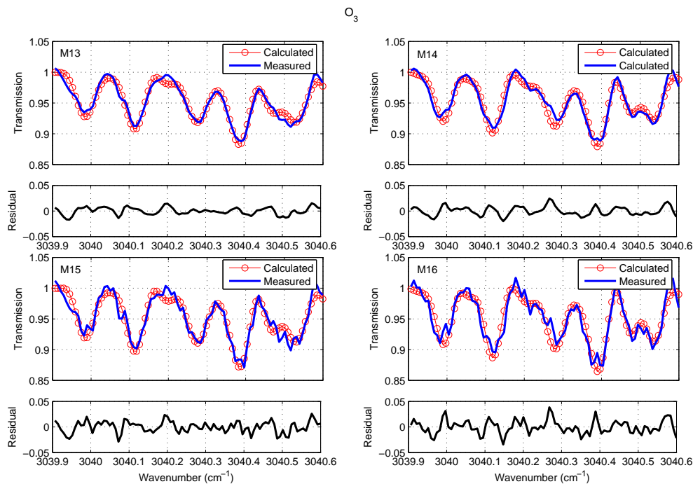
Figure 5.5: As in Figure 5.4, but for MCT O_3 spectral fits.
