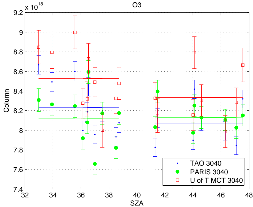
Figure 5.55: O 3 column amounts retrieved in the 3040 cm -1 microwindow as a function of solar zenith angle, using the parameters listed in Table 5.13. The horizontal lines show the means of the columns over the SZA range indicated. The error bars include the smoothing error, interference error, and the retrieval error added in quadrature.
