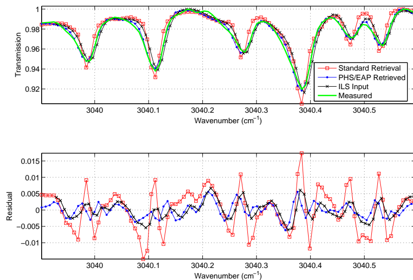
Figure 5.44: O 3 spectral fits for the U of T FTS (upper panel), and the residuals between the measured retrieval and the spectral fits (lower panel).
