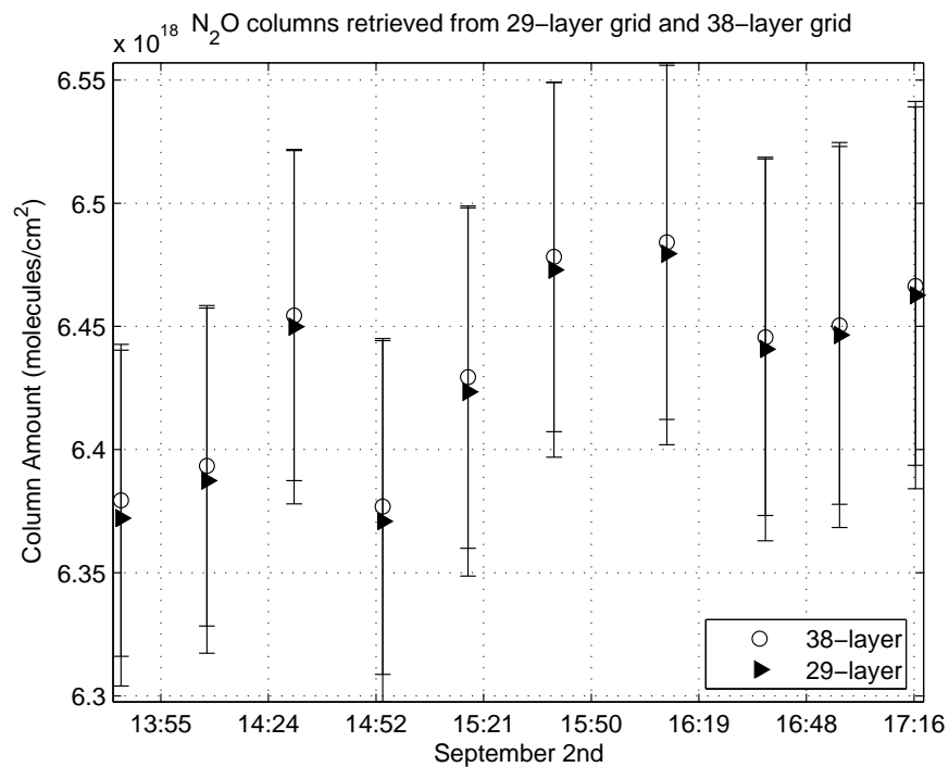
Figure 5.53: \text{N}_2\text{O} columns retrieved for 38- and 29-grid layers for PARIS-IR.
