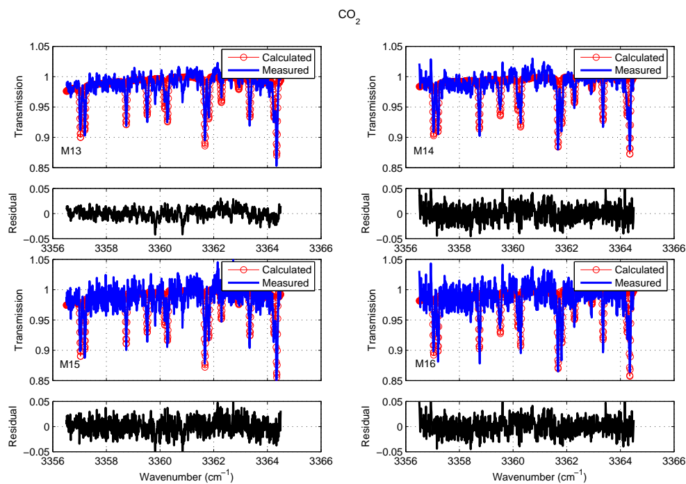
Figure 5.7: As in Figure 5.4, but for MCT \text{CO}_2 spectral fits.
