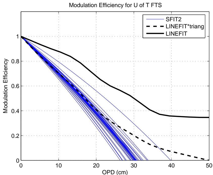
Figure 5.37: Comparison between EAP from SFIT2 and LINEFIT modulation efficiency. The LINEFIT modulation efficiency multiplied by the triangular function (dashed line) is used as the input to SFIT2 for this intercomparison.
