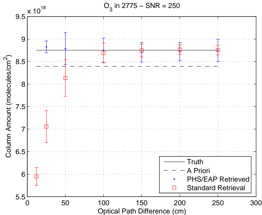
Figure 5.39: Simulated retrievals of ozone columns in the 2775\text{ cm}^{-1} microwindow, assuming \text{SNR}=250 , as a function of OPD. The small error bars on the PHS/EAP retrieval for 25 cm OPD are due to the small number of retrievals that converged for this OPD. The error bars are, as a consequence, not representative of the true standard deviation.
