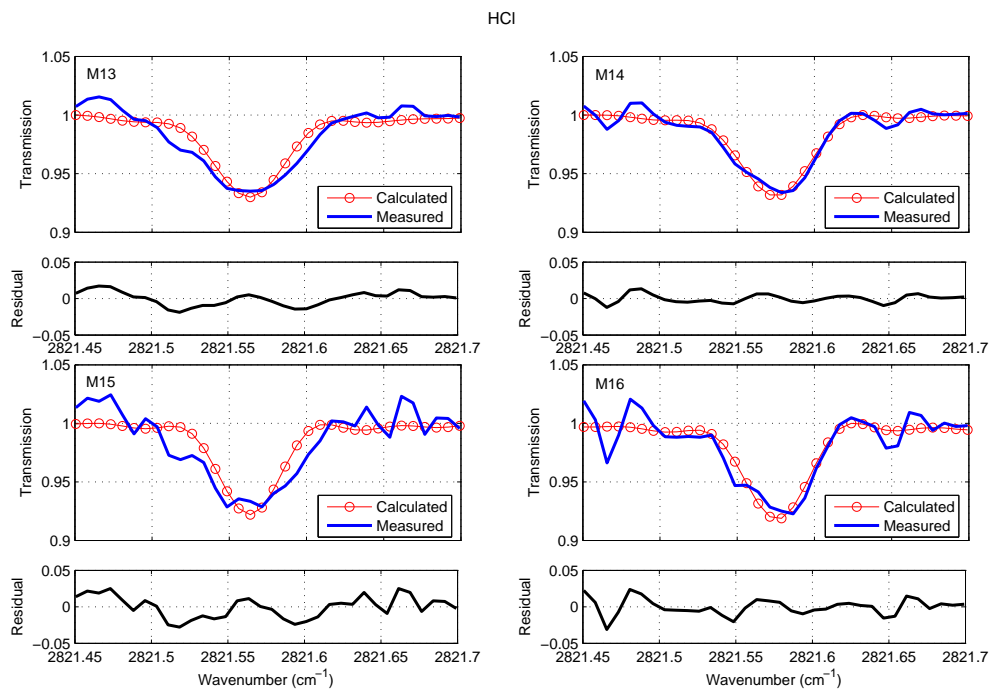
Figure 5.9: As in Figure 5.4, but for MCT HCl spectral fits. Only the first bandpass fit is shown.
