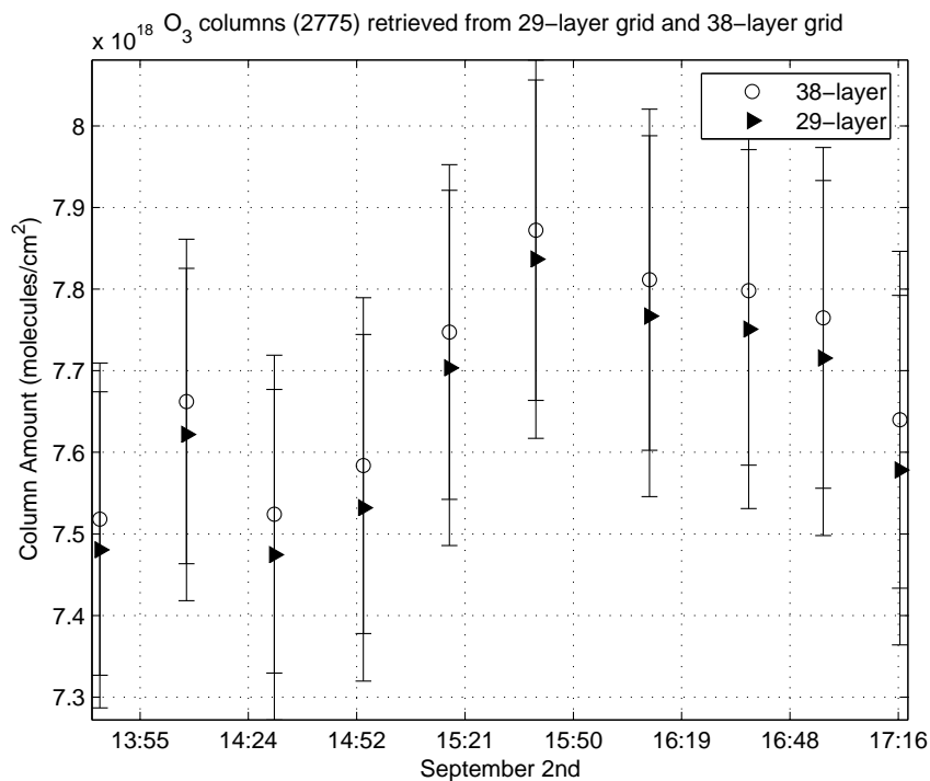
Figure 5.51: \text{O}_3 columns retrieved for 38- and 29-grid layers for PARIS-IR.
