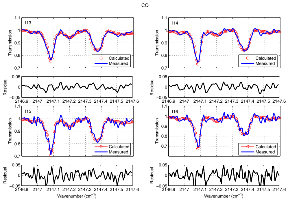
Figure 5.10: As in Figure 5.4, but for InSb CO spectral fits.
