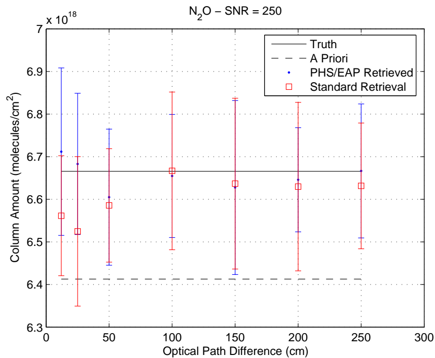
Figure 5.41: Simulated retrievals of N₂O columns, assuming SNR=250, as a function of OPD.
