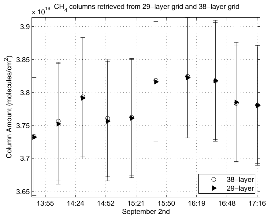
Figure 5.54: \text{CH}_4 columns retrieved for 38- and 29-grid layers for PARIS-IR.
