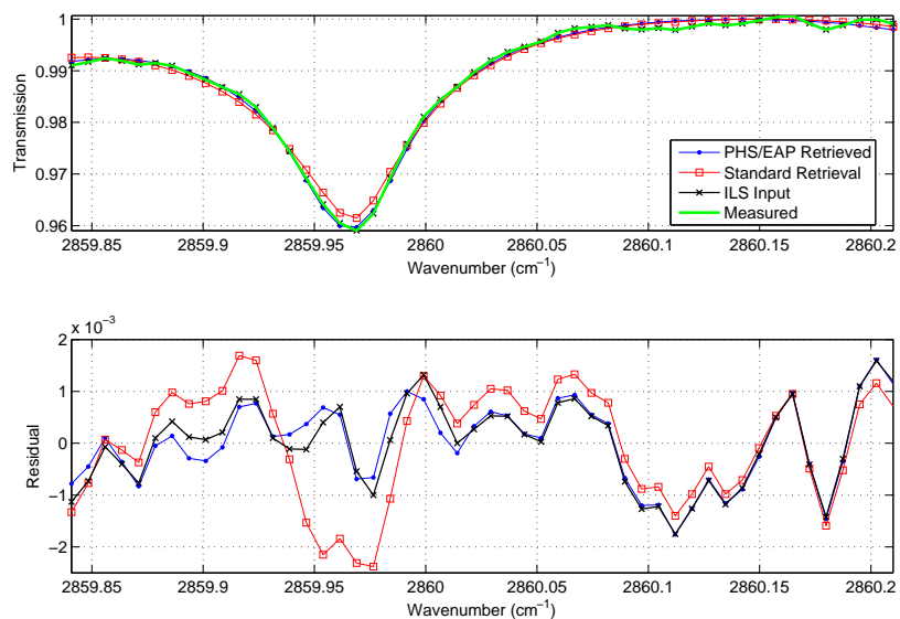
Figure 5.47: CH 4 spectral fits for the first CH 4 bandpass of the U of T FTS (upper panel), and the corresponding residuals (lower panel).
