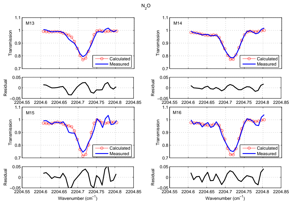
Figure 5.15: As in Figure 5.4, but for MCT \text{N}_2\text{O} spectral fits.
