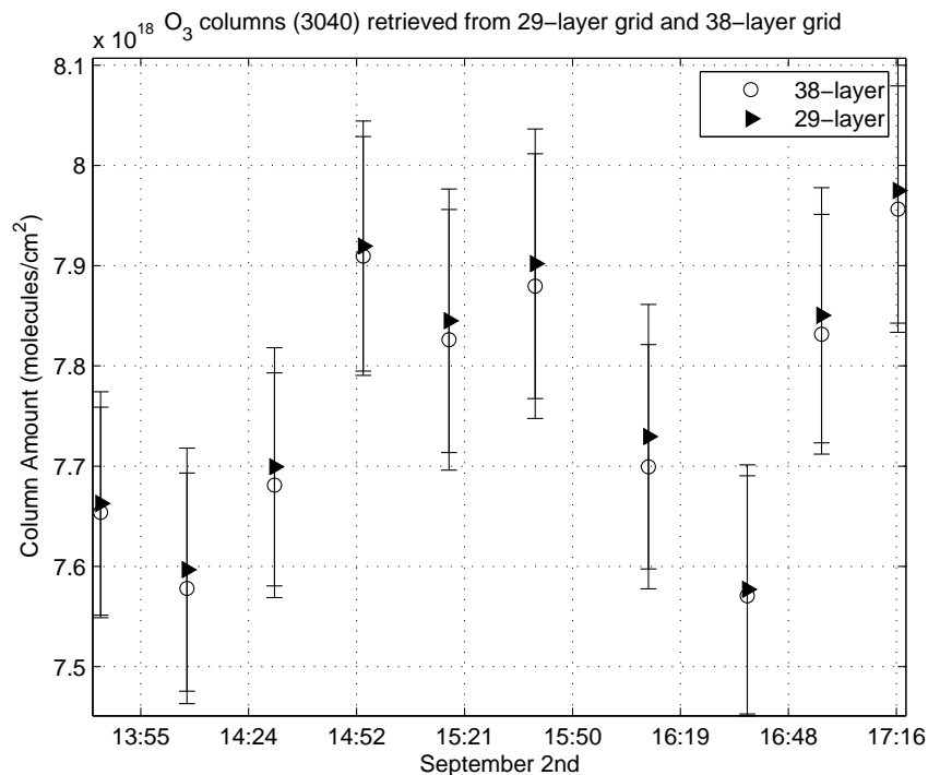
Figure 5.50: \text{O}_3 columns retrieved for 38- and 29-grid layers for PARIS-IR.
