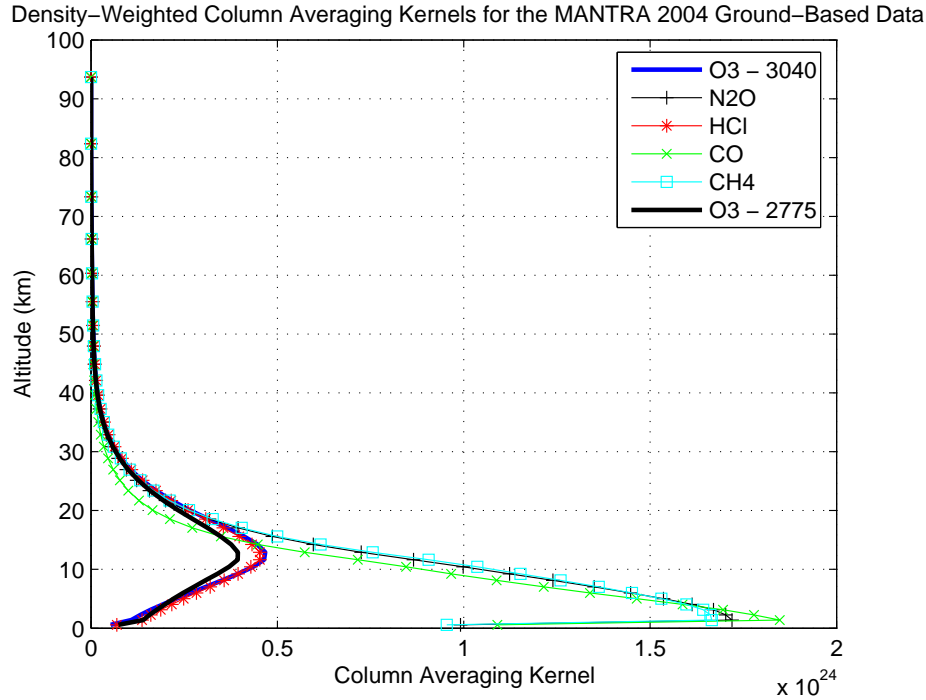
Figure 5.23: Density-weighted column averaging kernels for the U of T FTS ground-based data.
