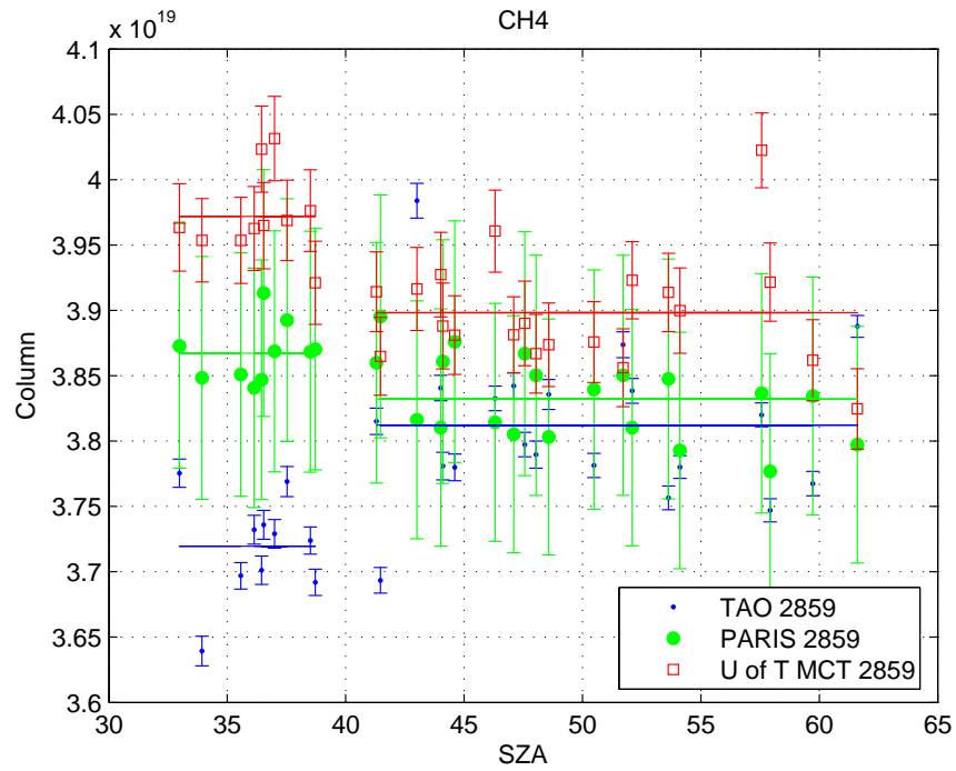
Figure 5.59: As in Figure 5.55, but for \text{CH}_4 .
