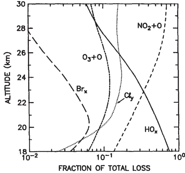
Figure 1.1: Fraction of total ozone loss at midlatitudes ( 47^\circ ) by the individual catalytic cycles. Figure reproduced from McElroy et al. [8].
