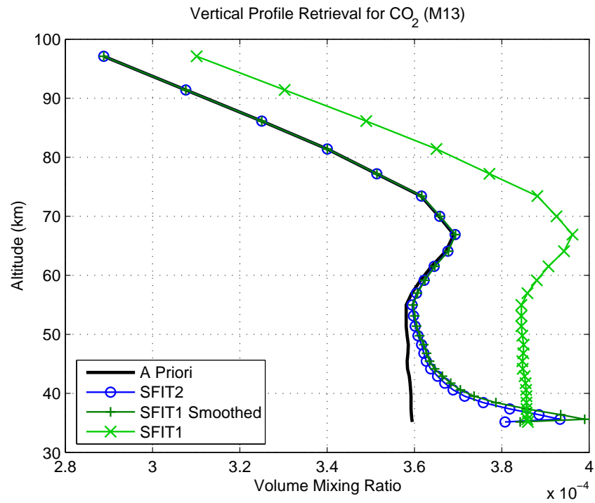
Figure 5.20: The SFIT2, original and smoothed SFIT1 \text{CO}_2 from the MANTRA 2004 flight data.
