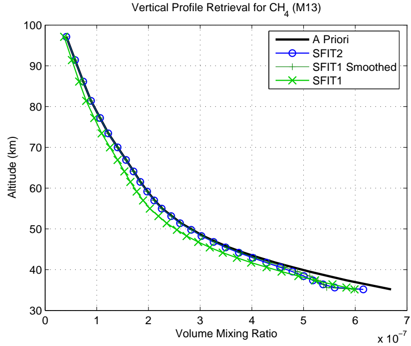
Figure 5.19: The SFIT2, original and smoothed SFIT1 \text{CH}_4 from the MANTRA 2004 flight data.
