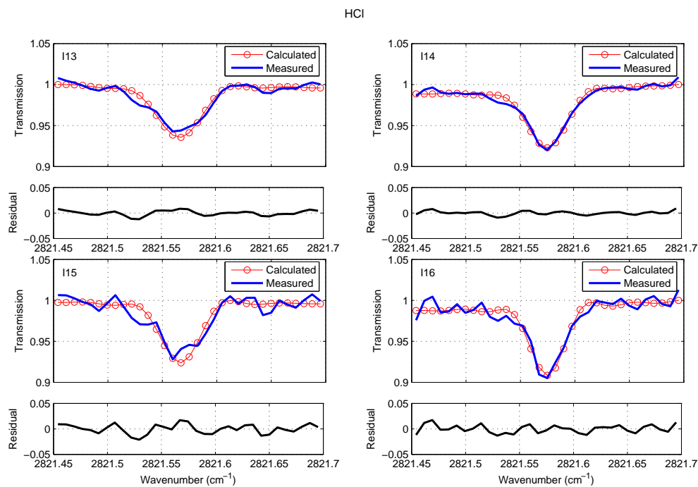
Figure 5.8: As in Figure 5.4, but for InSb \text{HCl} spectral fits. Only the first bandpass fit is shown.
