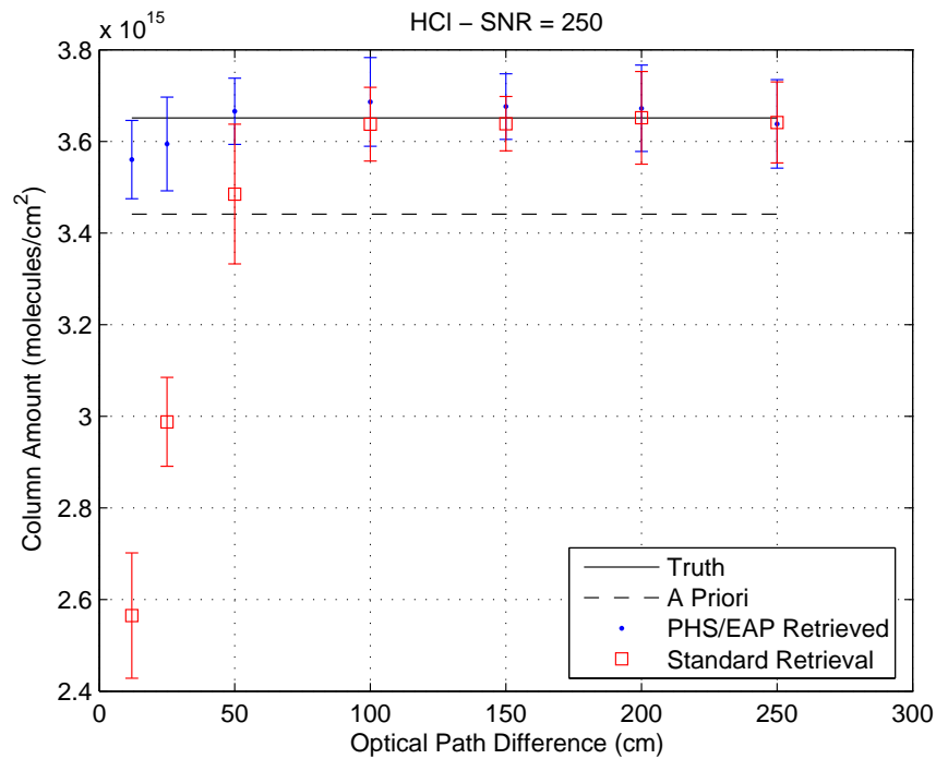
Figure 5.40: Simulated retrievals of HCl columns, assuming SNR=250, as a function of OPD.
