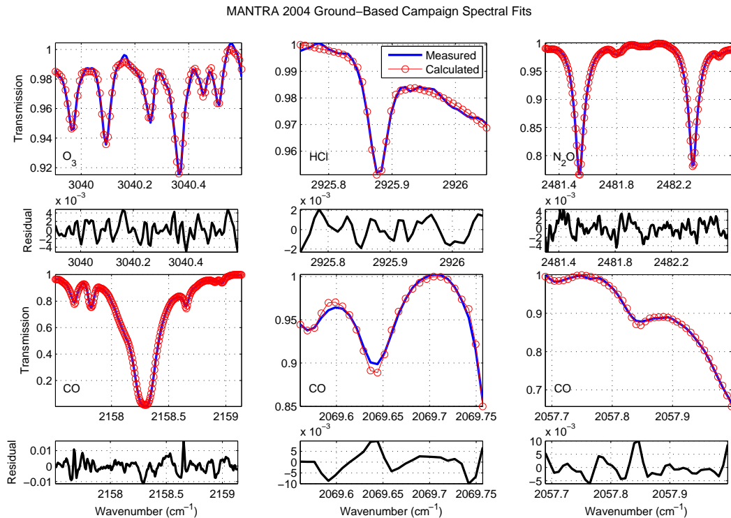
Figure 5.24: Representative examples of MCT spectral fits for the MANTRA 2004 ground-based data.
