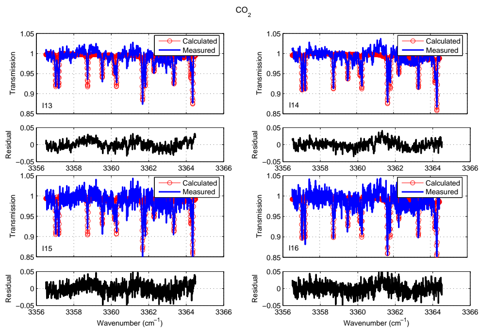
Figure 5.6: As in Figure 5.4, but for InSb CO_2 spectral fits.
