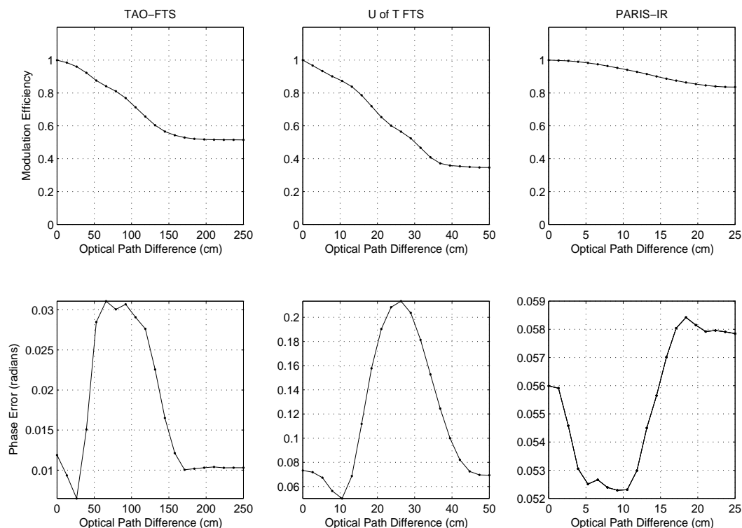
Figure 5.34: Typical modulation efficiency and phase error for all three instruments. These are computed from gas cell measurements using LINEFIT. The top panels contain the modulation efficiency and the lower panels contain the phase error (note the different y-axis scales on the phase error plots). The left-most panels show unapodized TAO-FTS data, recorded August, 2005. The central panels show U of T FTS data, apodized with a triangular filter and recorded September, 2005. The right-most panels show unapodized PARIS-IR data, recorded August, 2005.
