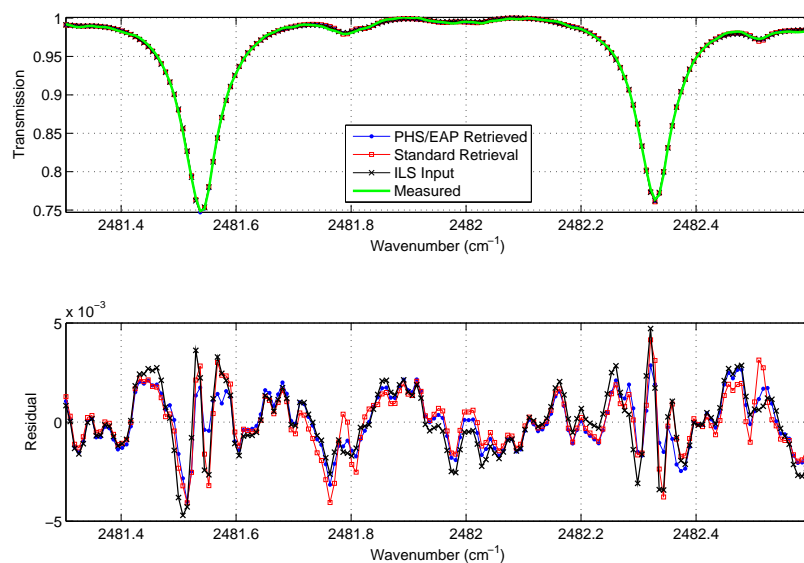
Figure 5.46: \text{N}_2\text{O} spectral fits for the U of T FTS (upper panel), and the corresponding residuals (lower panel).
