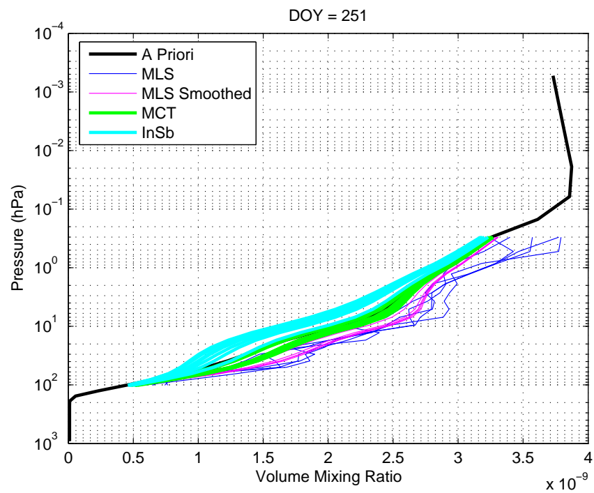
Figure 5.27: Partial profile comparisons as in Figure 5.25, but for HCl.
