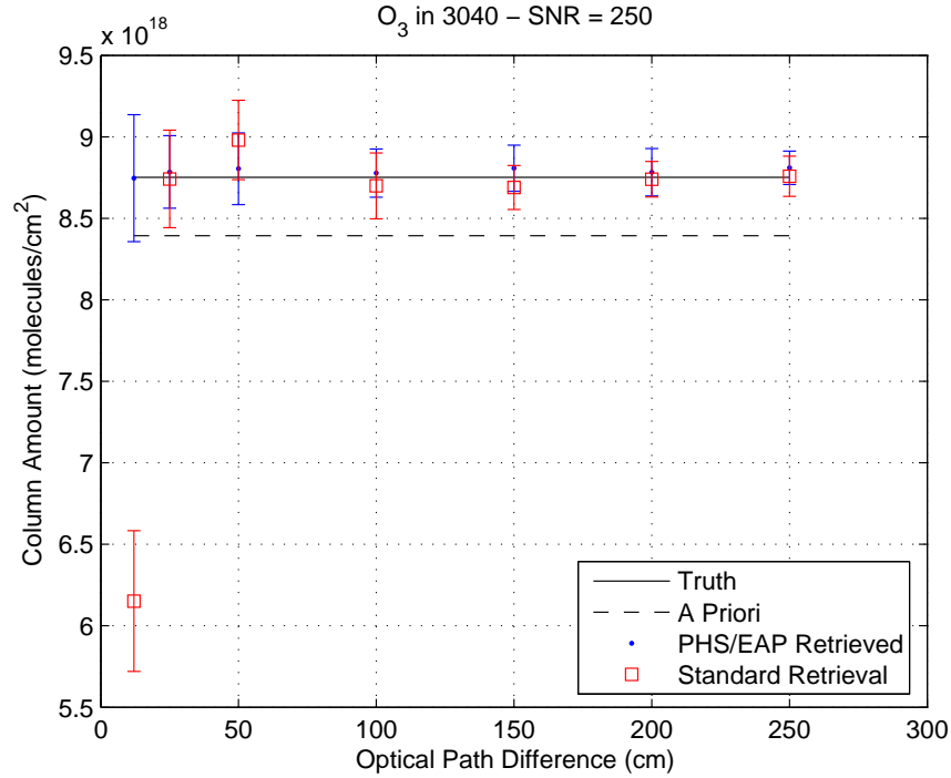
Figure 5.38: Simulated retrievals of ozone columns in the 3040\text{ cm}^{-1} microwindow, assuming \text{SNR}=250 , as a function of OPD.
