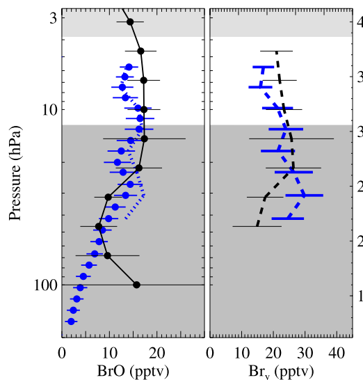
Figure 15. Same as Figure 14 except for BrO measurements obtained by the SAOZ-BrO instrument (blue) on 24 August 2004 at 52^\circ N . The MLS BrO error bars indicate a combination of precision and accuracy, and the SAOZ error bars indicate precision.
