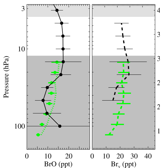
Figure 14. (left) Comparison of MLS day/night difference in BrO and (right) inferred Br_y with DOAS data from the 23 March 2003 flight at 68^\circ N . In Figure 14 (left), the black points show the MLS BrO day/night difference averaged over all days (149) retrieved with v2.2 as of the writing of this manuscript, from 55^\circ S to 55^\circ N . Both the MLS BrO error bars and the DOAS error bars [Dorf et al., 2006a] indicate a combination of precision and accuracy. The average solar zenith angle of the MLS measurements is 40^\circ . The nonshaded region indicates where the day/night difference in MLS BrO is representative of the daytime BrO. The lightly shaded region indicates where the day/night difference in MLS measurements of BrO is not representative of the daytime BrO; rather, one needs to take account of the nonnegligible nighttime BrO, which we have not done here. The darker shaded region indicates where MLS measurements of BrO are not suitable for scientific use. The green points show DOAS BrO, while the green dotted curve shows that data scaled using a photochemical model to a SZA of 65^\circ , the smallest SZA attained in March at that latitude. In Figure 14 (right), the dashed black curve is Br_y inferred from MLS BrO using a photochemical model. The dashed green curve shows Br_y similarly inferred from DOAS BrO. The error bars on the Br_y profiles indicate uncertainty due to measured BrO and NO_2 , as well as uncertainty in the model kinetics.
