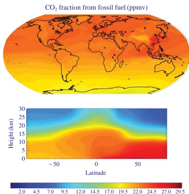
Fig. 6. The column-averaged CO 2 fraction (unit: ppmv) contributed by fossil fuel combustion and cement production from a tagged GEOS-Chem simulation for January 2004 and December 2009.
