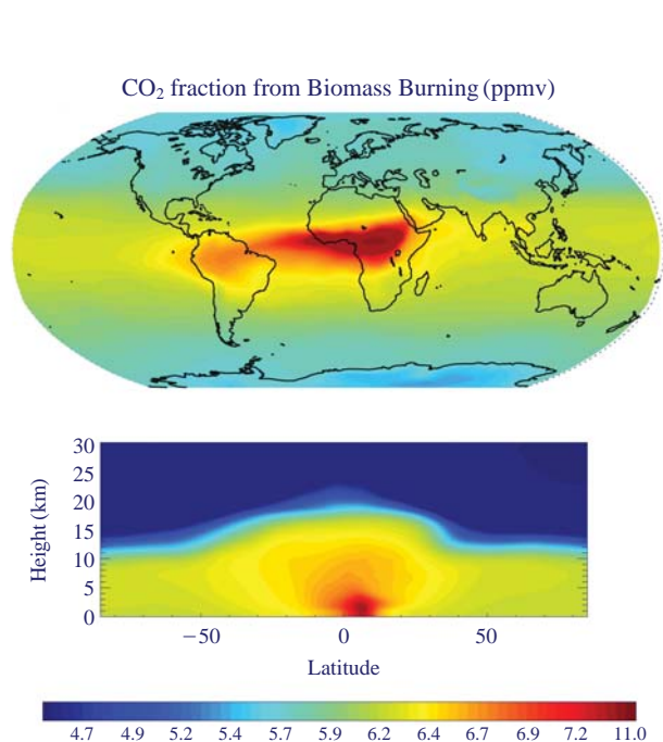
Fig. 7. Same as Fig. 6, but for the contribution from biomass burning.
