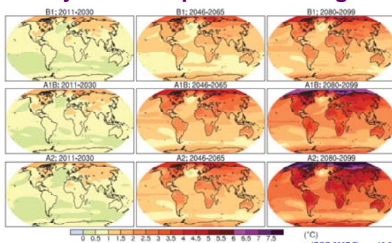
Figure 10.8. Multi-model mean of annual mean surface warming (surface air temperature change, °C) for the scenario B1 (top), A1B (middle) and A2 (bottom), and three time periods, 2011 to 2030 (left), 2046 to 2065 (middle) and 2080 to 2099 (right). Shading is omitted for clarity (see text). Anomalies are relative to the average of the period 1980 to 1999. Results for individual models can be seen in the Supplementary Material for this chapter.
