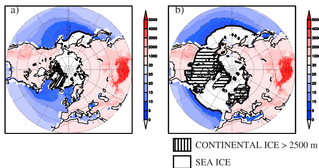
Figure 1. Northern Hemisphere planetary topographic height [m], SST [°C] and ice cover. Values smaller than 30 pertain to SST and larger than 30 to topographic height. The panel (a) for MOD simulation and (b) for LGM simulation. Ice on the surface of the continents is specified according to the ICE-4G model [Peltier, 1994].
