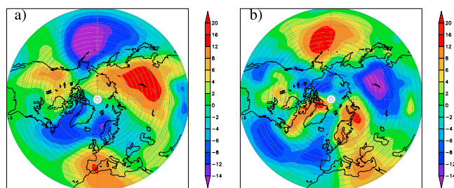
Figure 2. Distribution of eddy mean sea level pressure [hPa] (i.e., the sea level pressure with the zonal mean removed) in winter (DJF) for MOD simulation (a). (b) is the respective anomalies between the LGM and MOD simulations.
