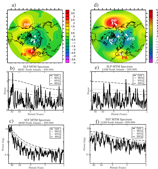
Figure 3. Leading EOF of SLP anomalies in DJF in the North Atlantic sector (20°–90°N, 90°W–40°E) for the MOD simulation (a) and the LGM simulation (d). The patterns are displayed as amplitudes (hPa) by regressing hemispheric SLP anomalies upon the standardized first principal component time series. Please note that Figures 3a and 3d are shown with distinct labels. PI, PA, PS and PP are the main centres of action over Iceland, Azores, Siberia and the North Pacific, respectively. (b) and (e) are the MTM power spectrum for the first PC of SLP in the MOD and LGM simulations. (c) and (f) are the same as in (b) and (d) but calculated for SST. Also shown is the corresponding confidence levels (smooth lines), 90%, 95% and 99% for significance relative to the null hypothesis (red noise).
