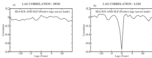
Figure 4. Lag correlation coefficient between the first PC of SLP and the correspond PC of sea-ice concentration for MOD simulation (a) and LGM simulation (b).
