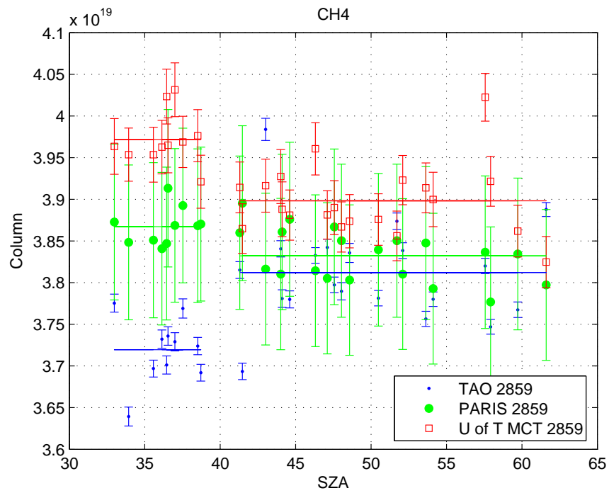
Figure 5.43: As in Figure 5.39, but for \text{CH}_4 .
