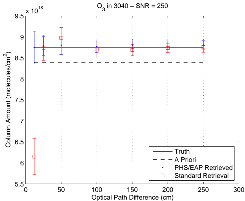
Figure 5.22: Simulated retrievals of ozone columns in the 3040\text{ cm}^{-1} microwindow, assuming \text{SNR}=250 , as a function of OPD.
