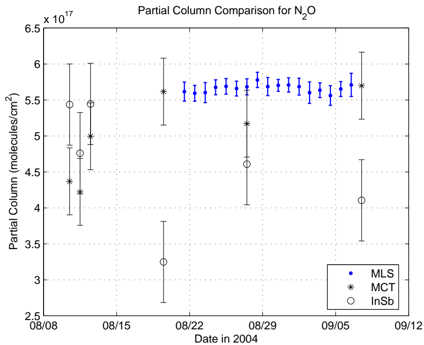
Figure 5.17: \text{N}_2\text{O} Partial Column Comparisons with MLS
