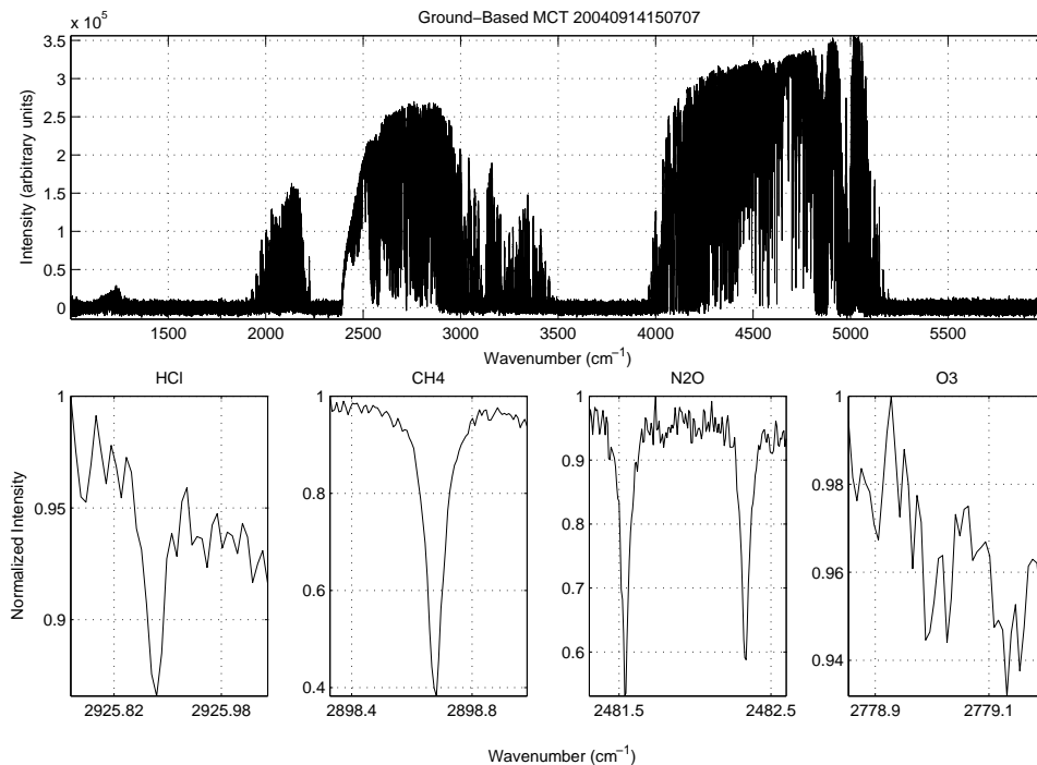
Figure 4.16: MCT Spectrum from the MANTRA 2004 Ground Based Campaign. The top panel shows the entire spectrum, while the lower four panels show microwindows from which we retrieve HCl, CH 4 , N 2 O and O 3 , respectively.
