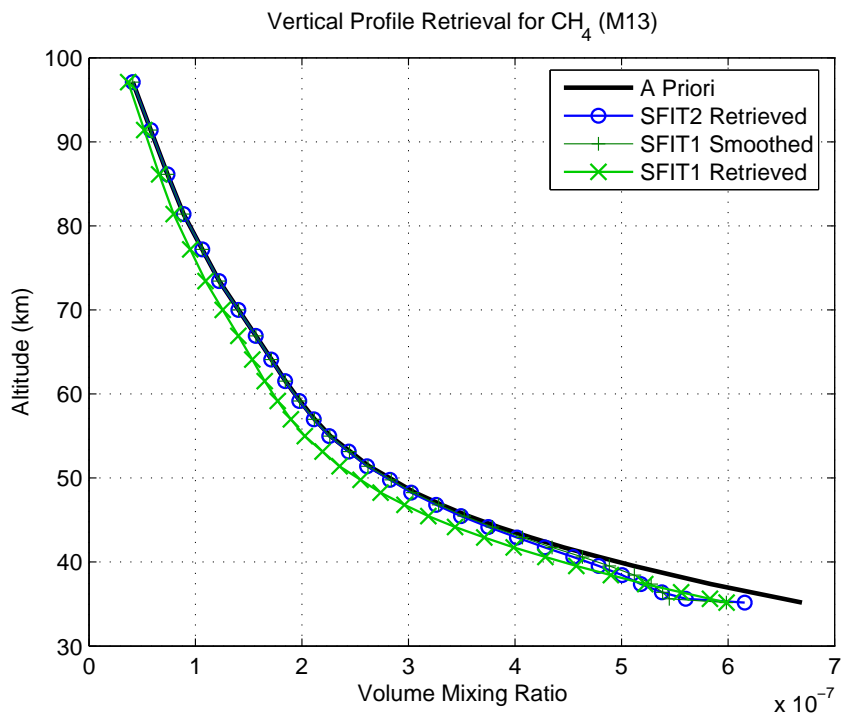
Figure 5.6: The SFIT2 and smoothed SFIT1 CH 4 from the MANTRA 2004 flight data.
