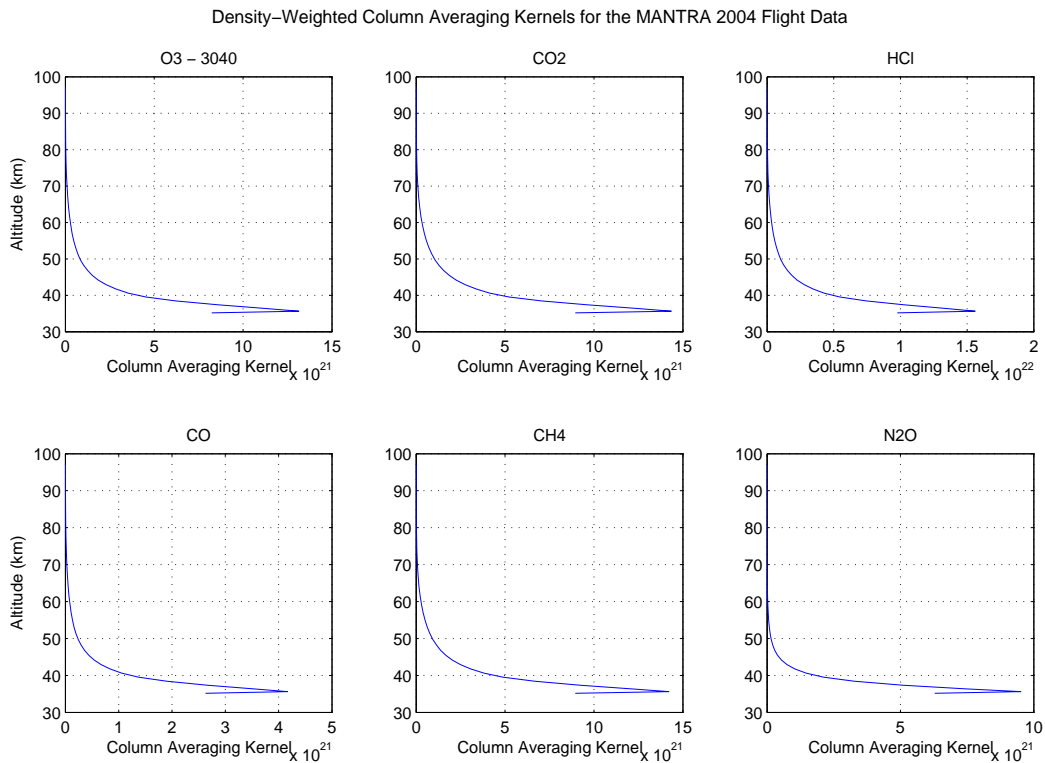
Figure 5.2: Flight Column Averaging Kernels
