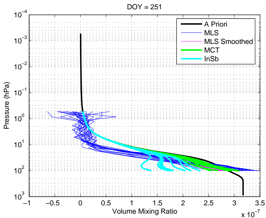
Figure 5.16: \text{N}_2\text{O} Partial Column Comparisons with MLS
