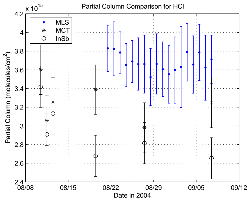
Figure 5.14: HCl Partial Column Comparisons with MLS
