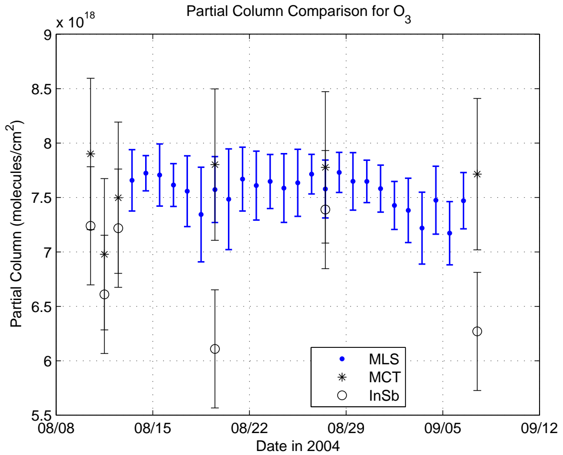
Figure 5.12: Ozone Partial Column Comparisons with MLS
