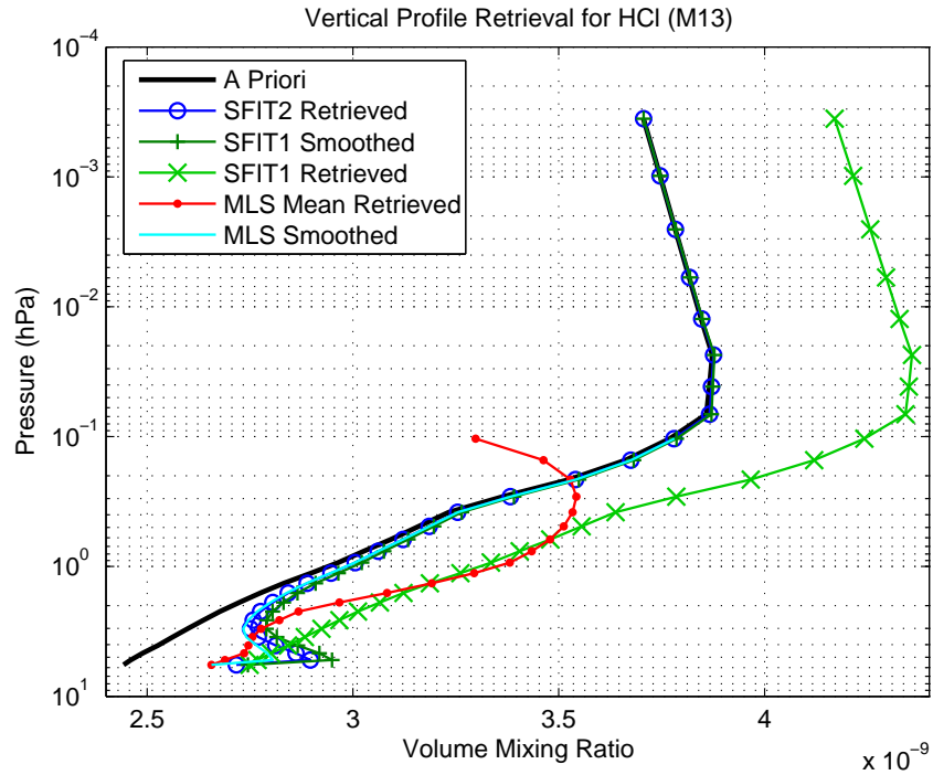
Figure 5.4: The SFIT2, smoothed SFIT1 and smoothed MLS mean HCl from the MANTRA 2004 flight data.
