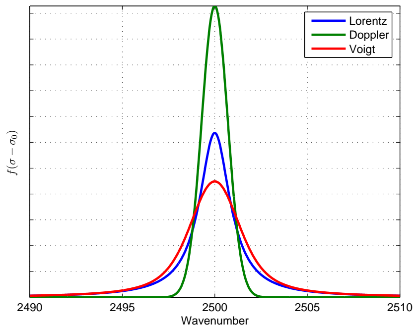
Figure 1.1: Doppler, Lorentz and Voigt lineshapes. The Doppler and Lorentz line shapes have 1 \text{ cm}^{-1} half-widths. The Voigt profile is a convolution of these Doppler and Lorentz line shapes.
