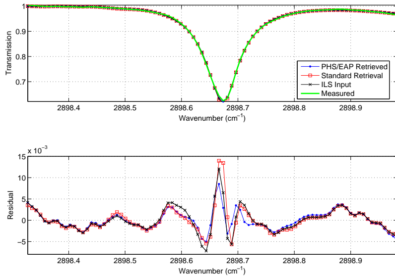
Figure 5.32: CH 4 spectral fits for the U of T FTS (upper panel), and the corresponding residuals (lower panel).
