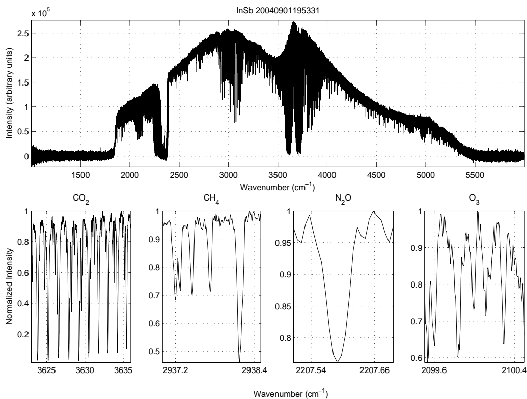
Figure 4.7: InSb Spectrum from MANTRA 2004 Flight 1
