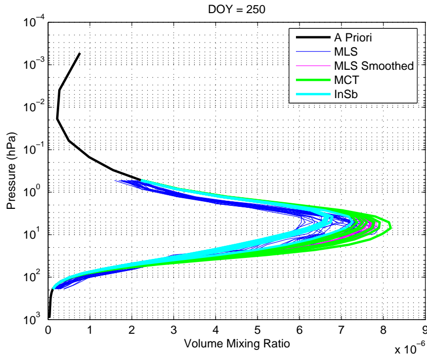
Figure 5.11: Ozone Partial Column Comparisons with MLS
