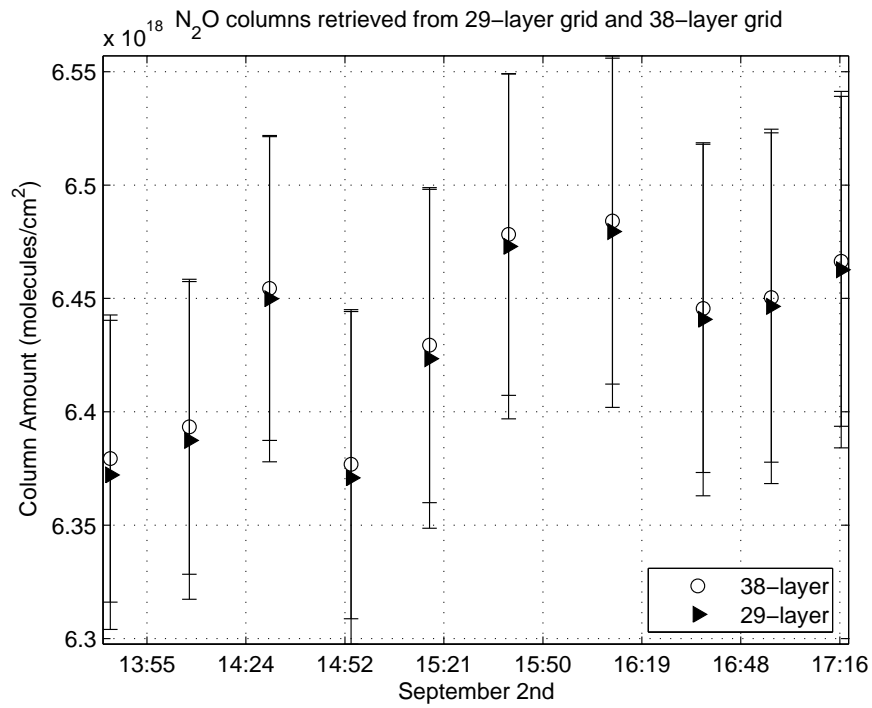
Figure 5.37: \text{N}_2\text{O} columns retrieved for 38- and 29-grid layers for PARIS-IR
