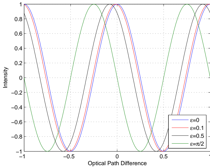
Figure 3.5: Cosine interferogram with different phase errors, \varepsilon .
