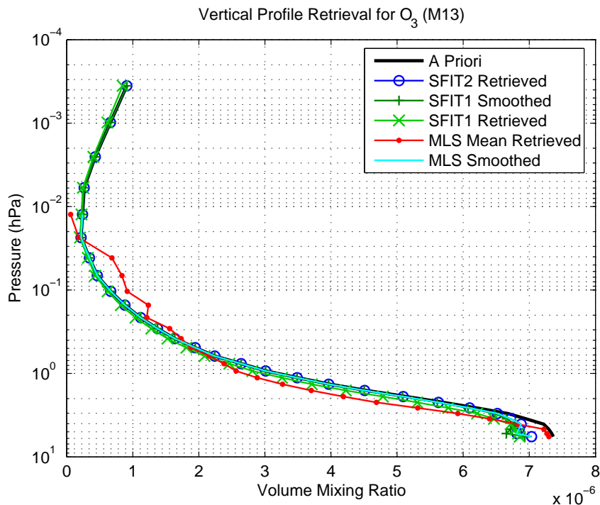
Figure 5.3: The SFIT2, smoothed SFIT1 and smoothed MLS mean ozone in the 3041 microwindow from the MANTRA 2004 flight data.
