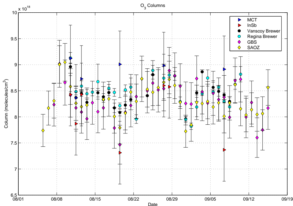
Figure 5.9: Daily Average Ozone for the MANTRA 2004 Ground-Based Campaign. The two detectors for the U of T FTS are in blue and red triangles. The black circles are from the Vanscoy Brewer, while the cyan circles are from the Regina Brewer. The diamonds are from the ground-based UV-VIS instruments: magenta is the University of Toronto Ground-Based Spectrometer and yellow is the SAOZ instrument.
