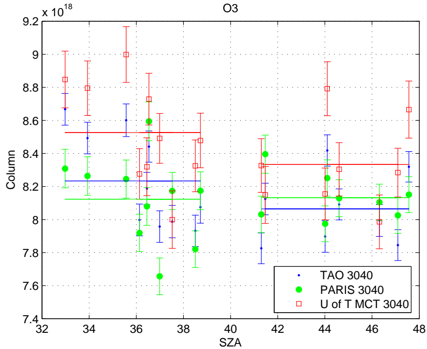
Figure 5.39: \text{O}_3 column amounts retrieved in the 3040 \text{ cm}^{-1} microwindow as a function of solar zenith angle, using the parameters listed in Table 5.11. The horizontal lines show the means of the columns over the SZA range indicated. The error bars include the smoothing error, interference error, and the retrieval error added in quadrature.
