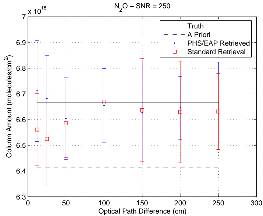
Figure 5.25: Simulated retrievals of N 2 O columns, assuming SNR=250, as a function of OPD.
