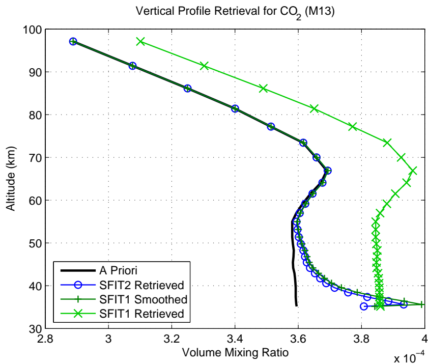
Figure 5.7: The SFIT2 and smoothed SFIT1 CO 2 from the MANTRA 2004 flight data.
