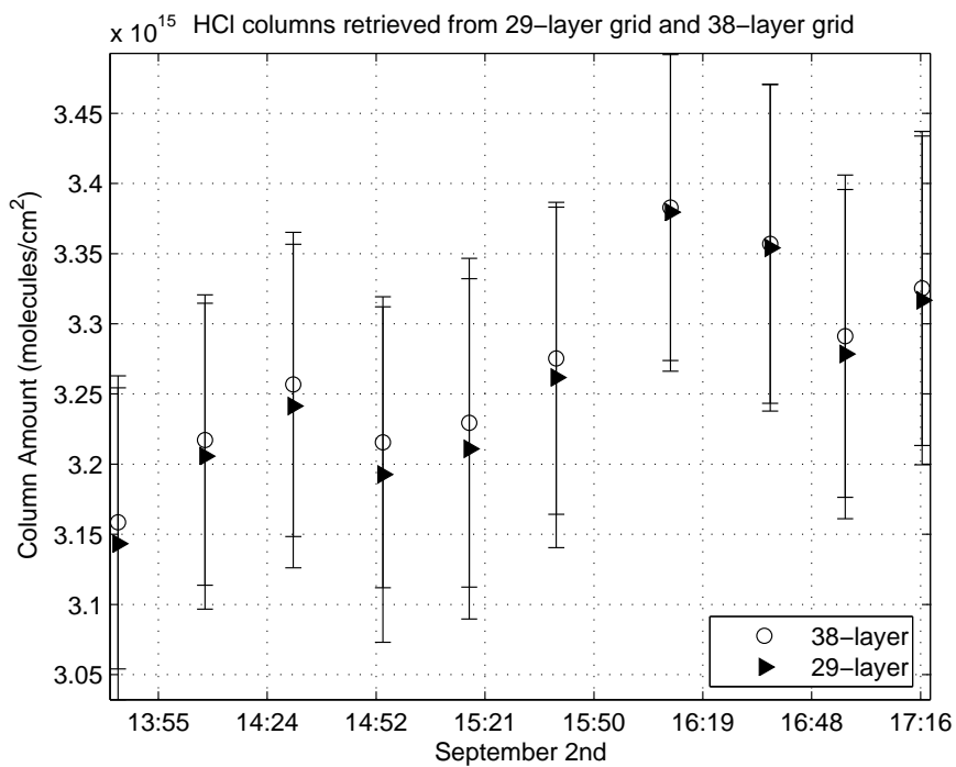
Figure 5.36: HCl columns retrieved for 38- and 29-grid layers for PARIS-IR
