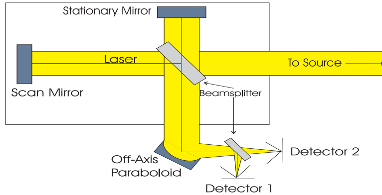
Figure 3.1: A schematic of a Fourier transform spectrometer.
