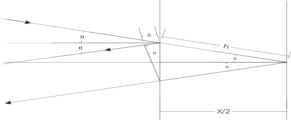
Figure 3.2: Extended source. The two vertical lines represent the two mirrors of the FTS, and so the path difference between them for an on-axis ray is x . Light enters from the top left at an angle \theta to the on-axis ray, which is subtended by the source of finite extent. The distance 2h - \delta is x_{eff} [52].
