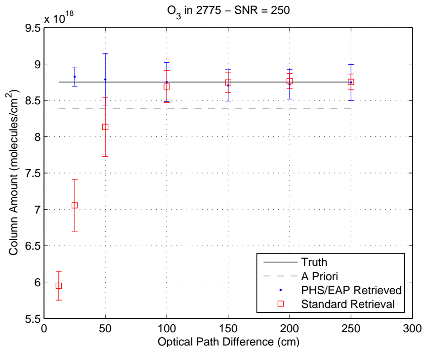
Figure 5.23: Simulated retrievals of ozone columns in the 2775\text{ cm}^{-1} microwindow, assuming \text{SNR}=250 , as a function of OPD. The small error bars on the PHS/EAP retrieval for 25 cm OPD are due to the small number of retrievals that converged for this OPD. The error bars are, as a consequence, artificially small.
