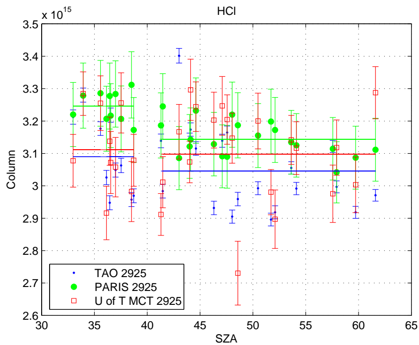
Figure 5.41: As in Figure 5.39, but for HCl.
