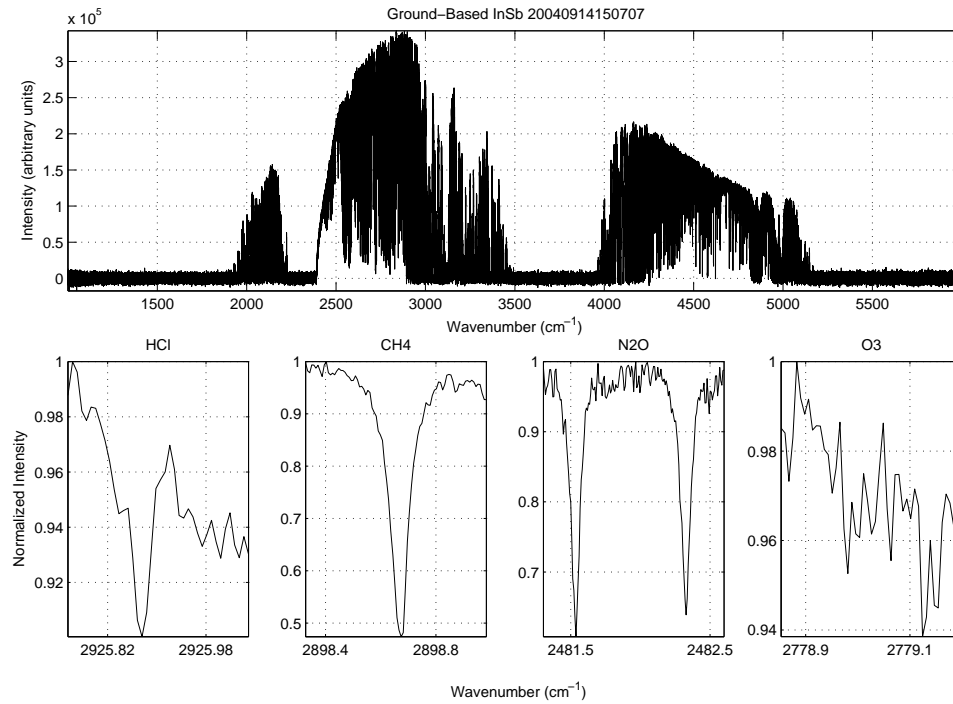
Figure 4.15: InSb Spectrum from the MANTRA 2004 Ground Based Campaign. The top panel shows the entire spectrum, while the lower four panels show microwindows from which we retrieve HCl, CH 4 , N 2 O and O 3 , respectively.
