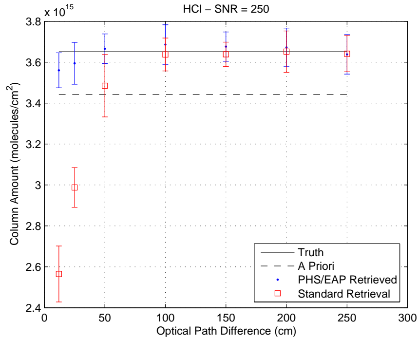
Figure 5.24: Simulated retrievals of HCl columns, assuming SNR=250, as a function of OPD.
