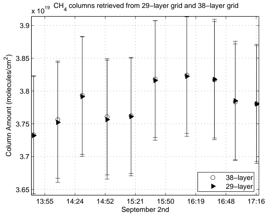
Figure 5.38: \text{CH}_4 columns retrieved for 38- and 29-grid layers for PARIS-IR
