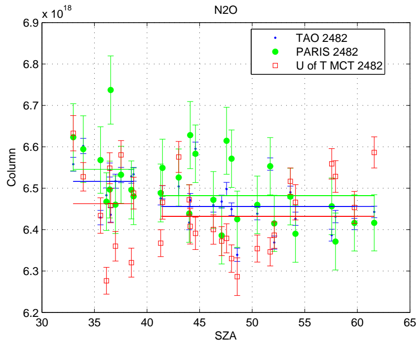
Figure 5.42: As in Figure 5.39, but for \text{N}_2\text{O} .
