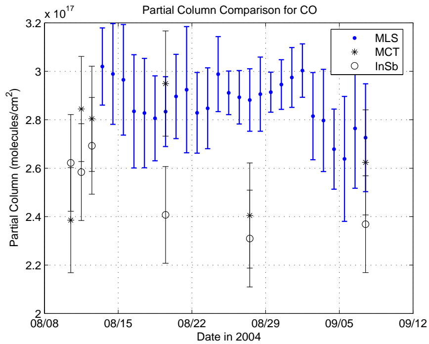
Figure 5.19: CO Partial Column Comparisons with MLS
