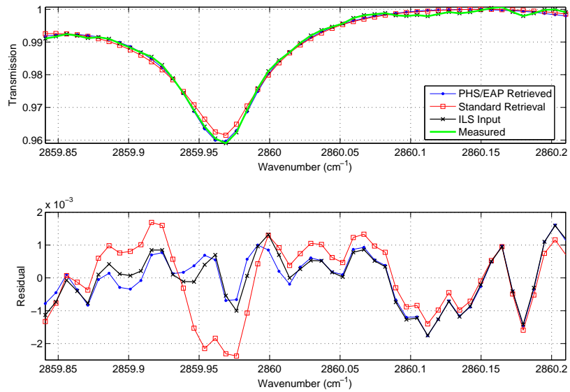
Figure 5.31: CH 4 spectral fits for the U of T FTS (upper panel), and the corresponding residuals (lower panel).
