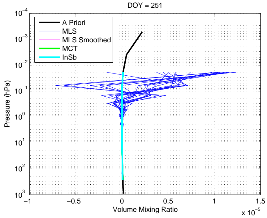
Figure 5.18: CO Partial Column Comparisons with MLS
