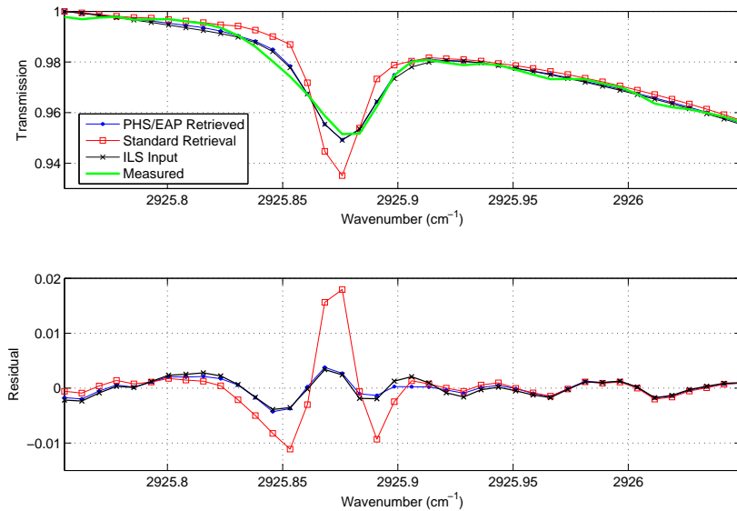
Figure 5.29: HCl spectral fits for the U of T FTS (upper panel), and the corresponding residuals (lower panel).
