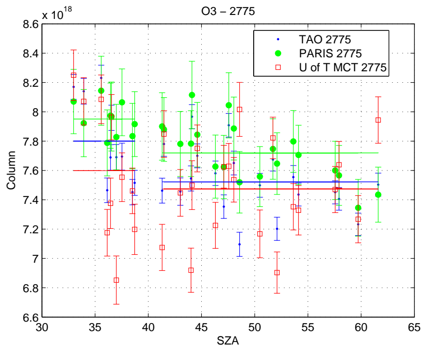
Figure 5.40: As in Figure 5.39, but for \text{O}_3 in the 2775 \text{ cm}^{-1} microwindow.
