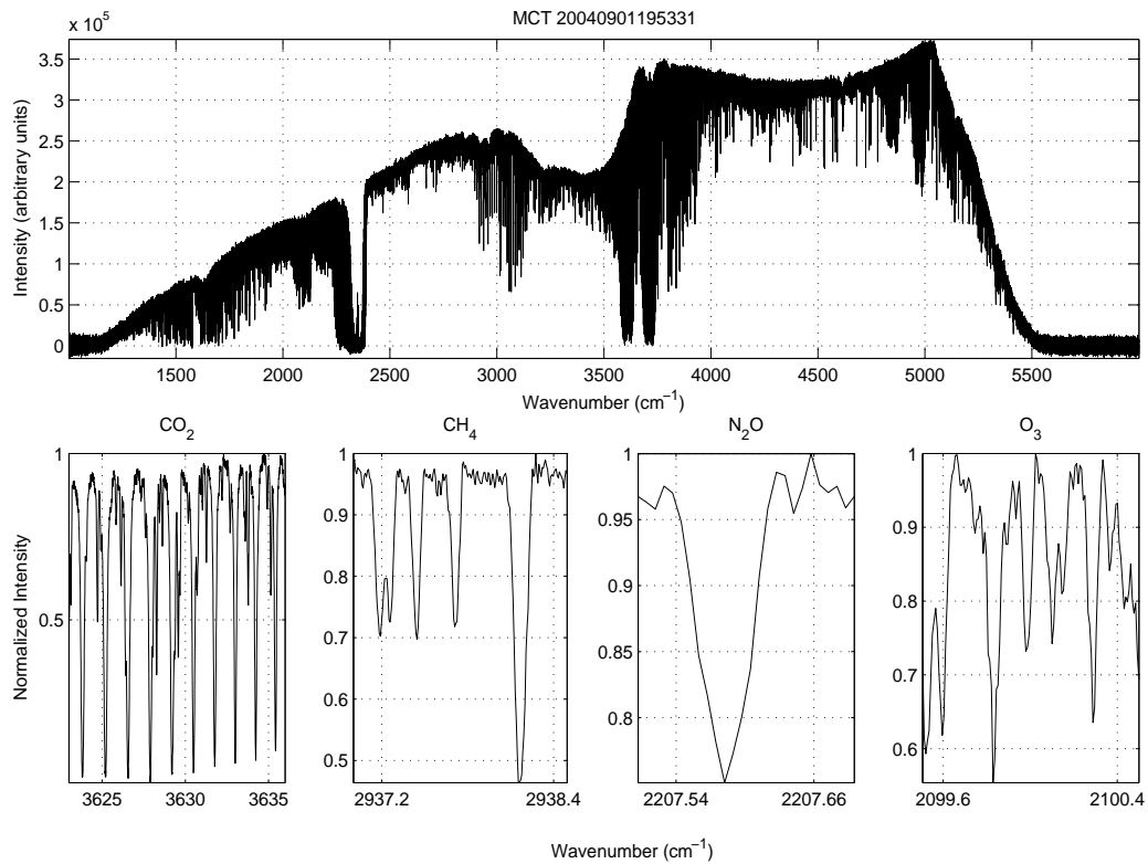
Figure 4.8: MCT Spectrum from MANTRA 2004 Flight 1
