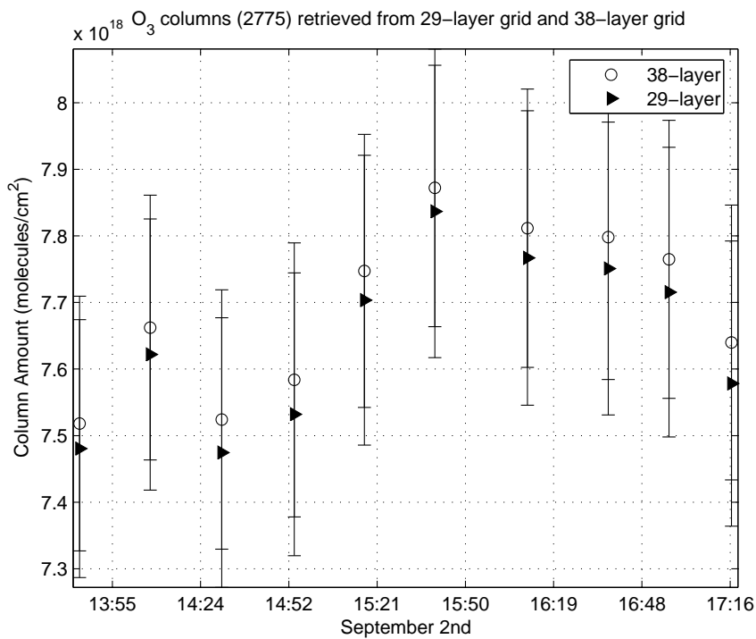
Figure 5.35: O 3 columns retrieved for 38- and 29-grid layers for PARIS-IR
