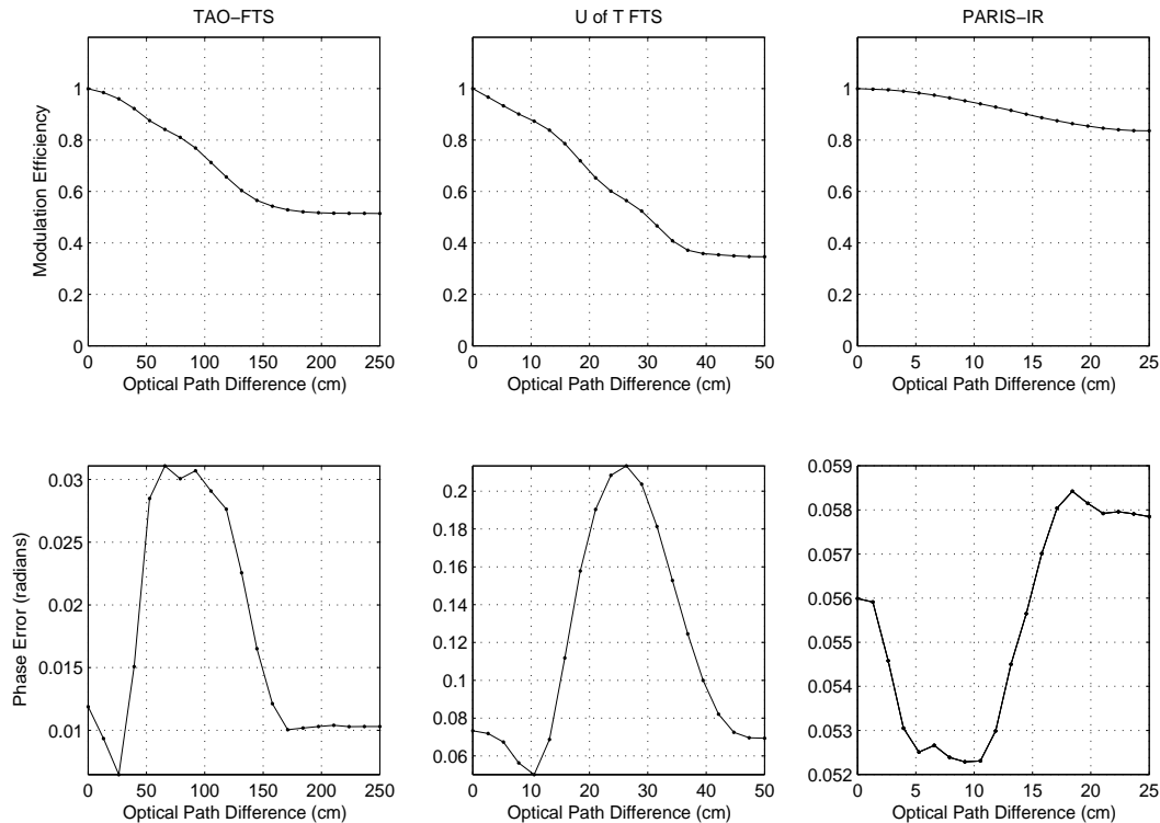
Figure 5.20: Typical modulation efficiency and phase error for all three instruments. These are computed from gas cell measurements using LINEFIT. The top panels contain the modulation efficiency and the lower panels contain the phase error. The left-most panels show unapodized TAO-FTS data, recorded August, 2005. The central panels show U of T FTS data, apodized with a triangular filter and recorded September, 2005. The right-most panels show unapodized PARIS-IR data, recorded August, 2005.
