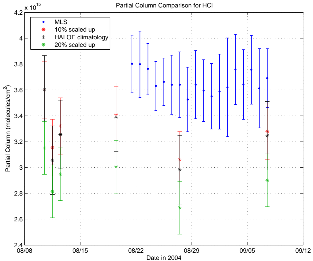
Figure 5.15: HCl Partial Column Comparisons with MLS. The different colours for the U of T FTS partial column data correspond to the different a priori profiles used to retrieve HCl partial columns, in an attempt to improve agreement between MLS and the U of T FTS.
