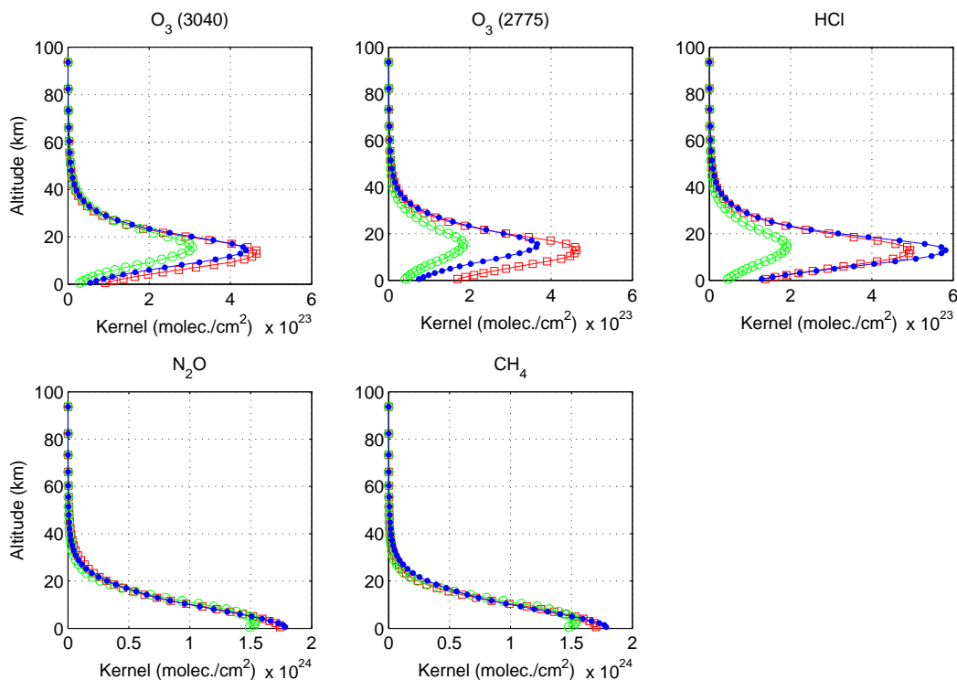
Figure 5.44: Density-weighted column averaging kernels for the three instruments: TAO-FTS (blue dots), U of T FTS (red squares) and the PARIS-IR (green circles), illustrating the sensitivity of the retrieved column at each altitude.
