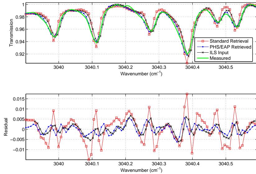
Figure 5.28: O 3 spectral fits for the U of T FTS (upper panel), and the residuals between the measured retrieval and the spectral fits (lower panel).
