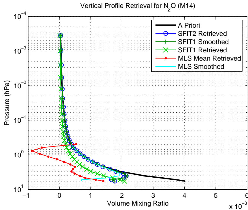
Figure 5.5: The SFIT2, smoothed SFIT1 and smoothed MLS mean N_2O from the MANTRA 2004 flight data.
