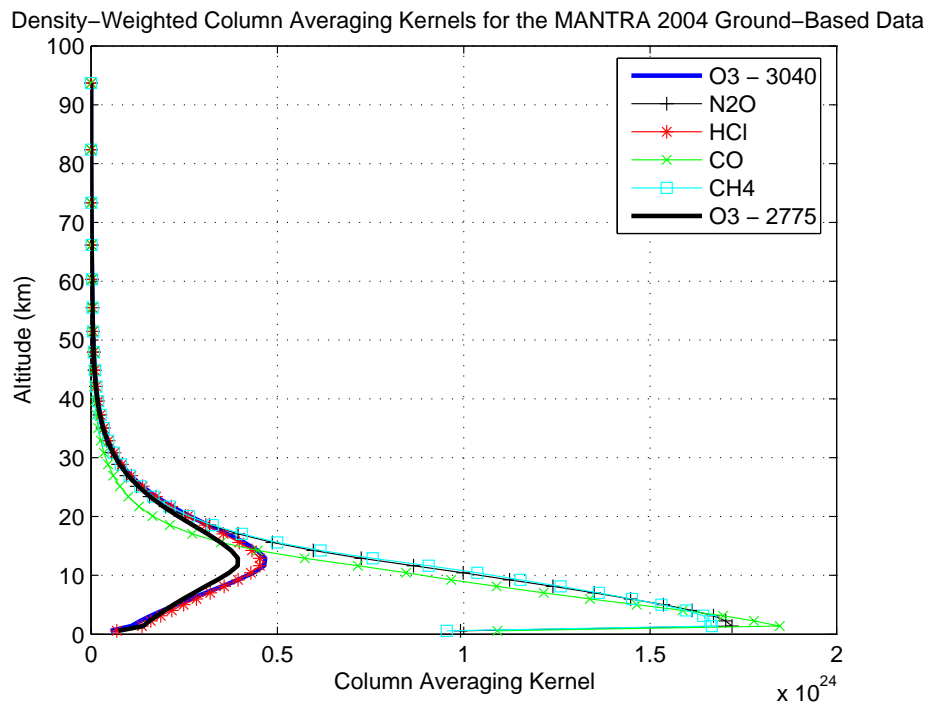
Figure 5.10: Density-Weighted Column Averaging Kernels for the U of T FTS Ground-Based Data
