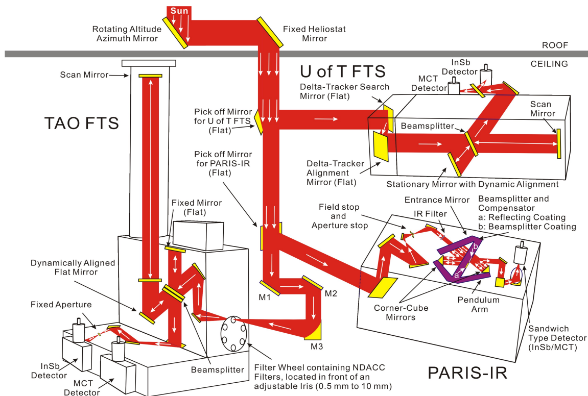
Figure 5.21: The experimental setup. Figure courtesy Dejian Fu.
