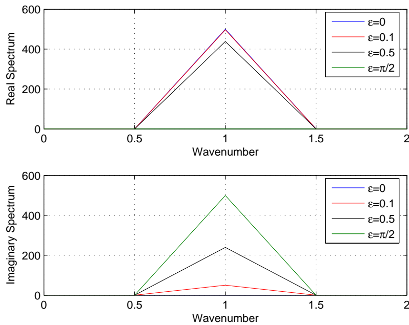
Figure 3.6: FFT of a cosine interferogram with different phase errors, \varepsilon . Note that the larger we make \varepsilon , the more information is transferred from the real part of the spectrum (top panel) to the imaginary part (lower panel), until we reach \pi/2 , when the cosine function becomes a sine function and all the information is now contained in the imaginary.
