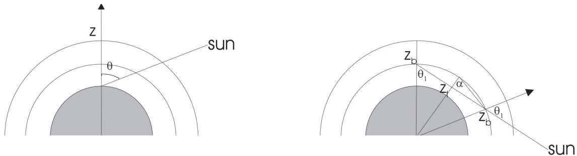
Figure 1.2: Ground-based (left panel) and balloon-based (right panel) viewing geometries.
