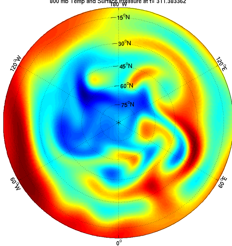
800 mb Temp and Surface Pressure at t= 311.383362
