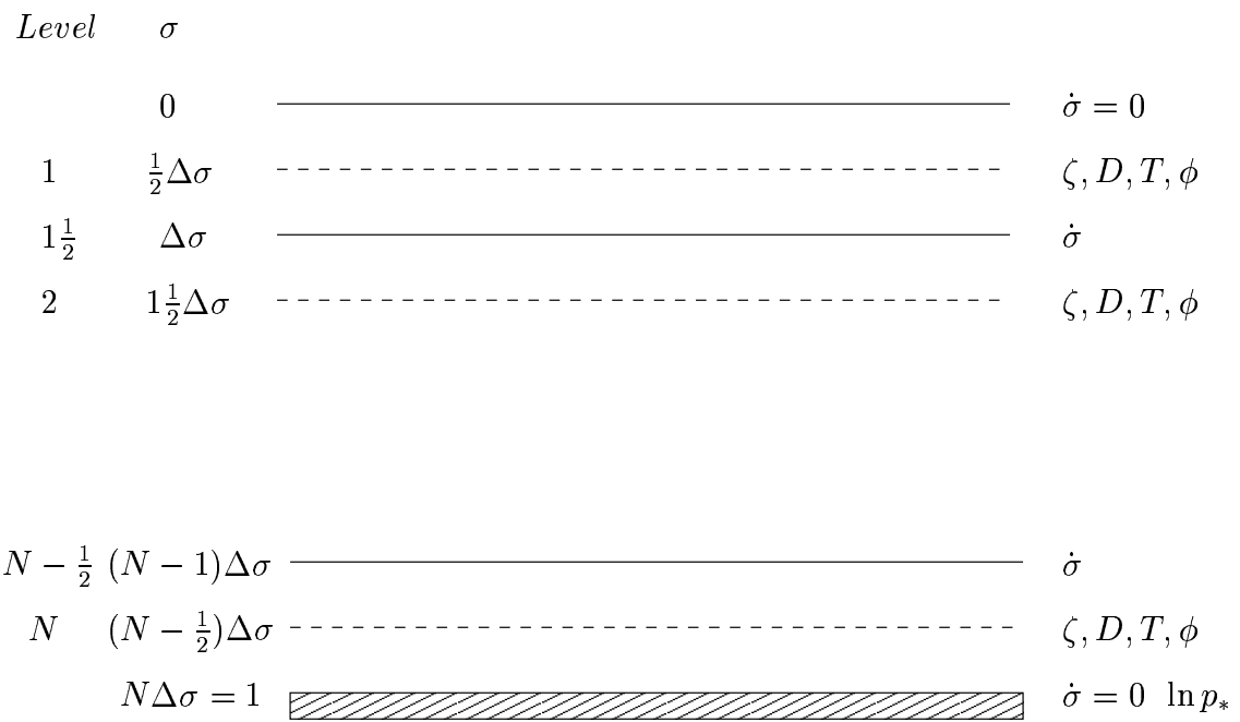
Figure 1: Vertical grid structure
