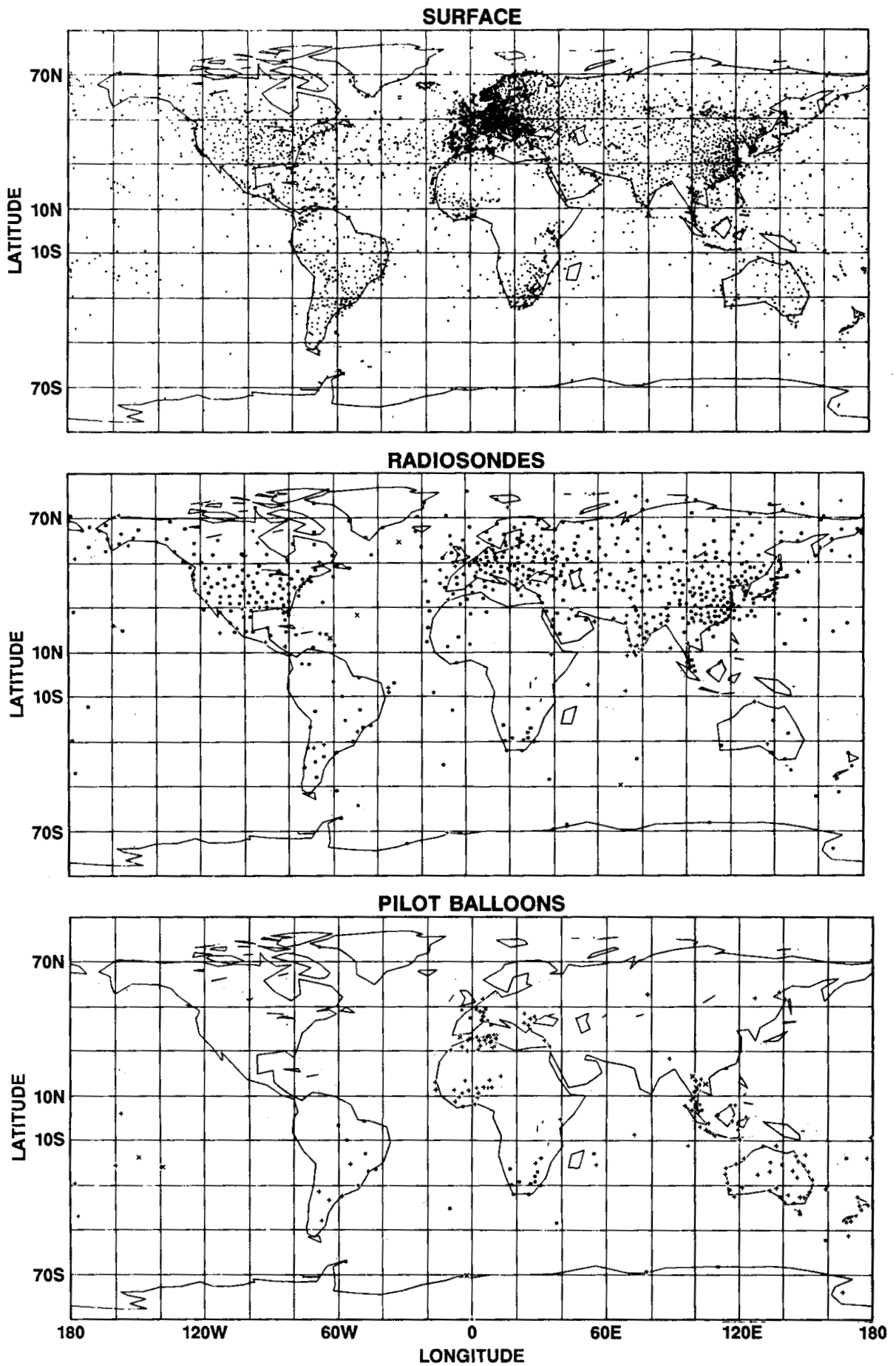
Figure 1.5 Global coverage map for various observing systems for the 6-hour period from 0900–1500 GMT 2 January 1989. (European Centre for Medium Range Forecasting.)
