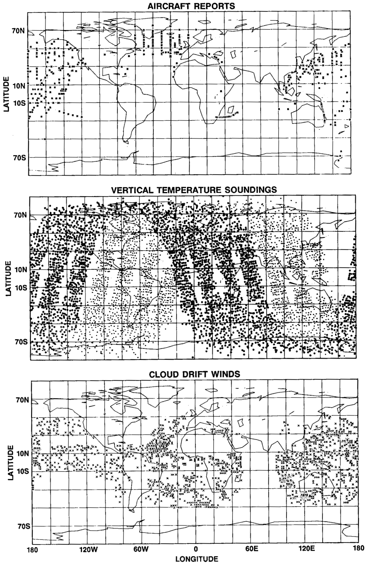
Figure 1.6 Same as Figure 1.5 but with different observing systems.
