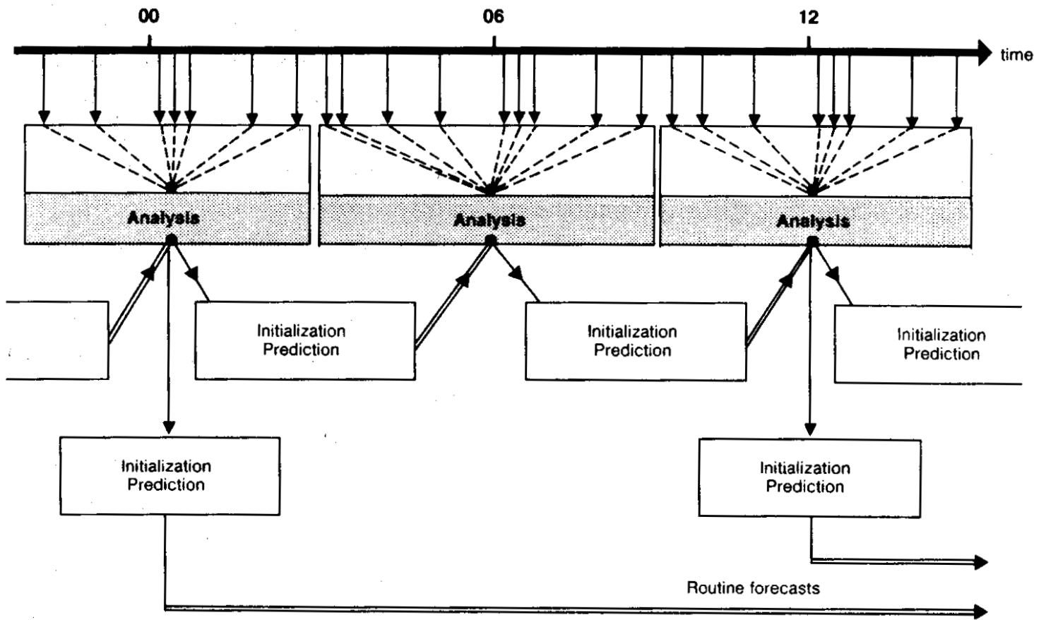
Figure 1.11 Schematic diagram of intermittent data assimilation cycle.
